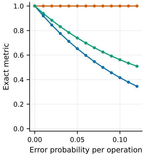
Qudit dephasing
