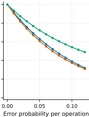
Qudit depolarization
