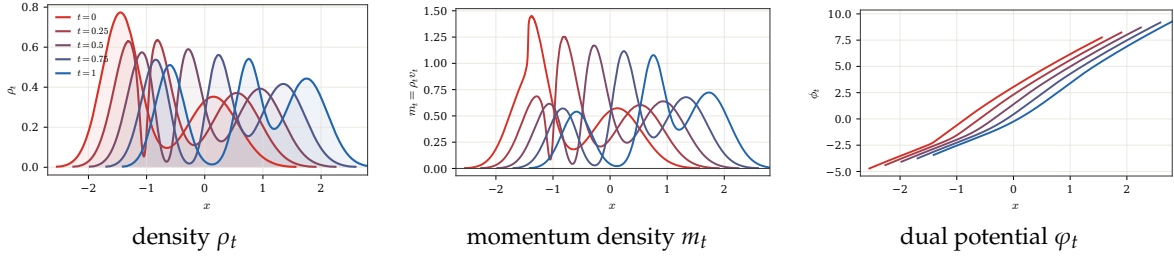
Figure 14.1: One-dimensional Benamou–Brenier primal and dual solutions. The endpoints are Gaussian mixtures and the solution is computed from monotone quantile interpolation. The left and middle panels show the primal density and the momentum density m_t = \rho_t v_t . The right panel shows the dual Hamilton–Jacobi potential, normalized up to an additive constant. Along the active transported mass, the notebook checks the primal–dual identities m_t = \rho_t \partial_x \varphi_t/2 and \partial_t \varphi_t + |\partial_x \varphi_t|^2/4 = 0 .
