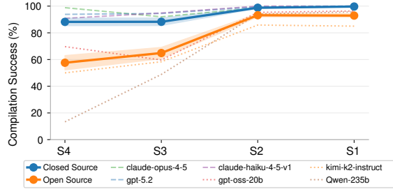
Figure 4. Code Execution Success Rate vs primitive abstraction. Increases, mirroring how prior Code-as-Policies (Liang et al., 2023) approaches relying on high-level primitives report strong zero-shot performance. By collapsing low-level perception, geometric reasoning, and control into human-designed primitives, these abstractions reduce the effective search space and allow models to focus on task sequencing.
