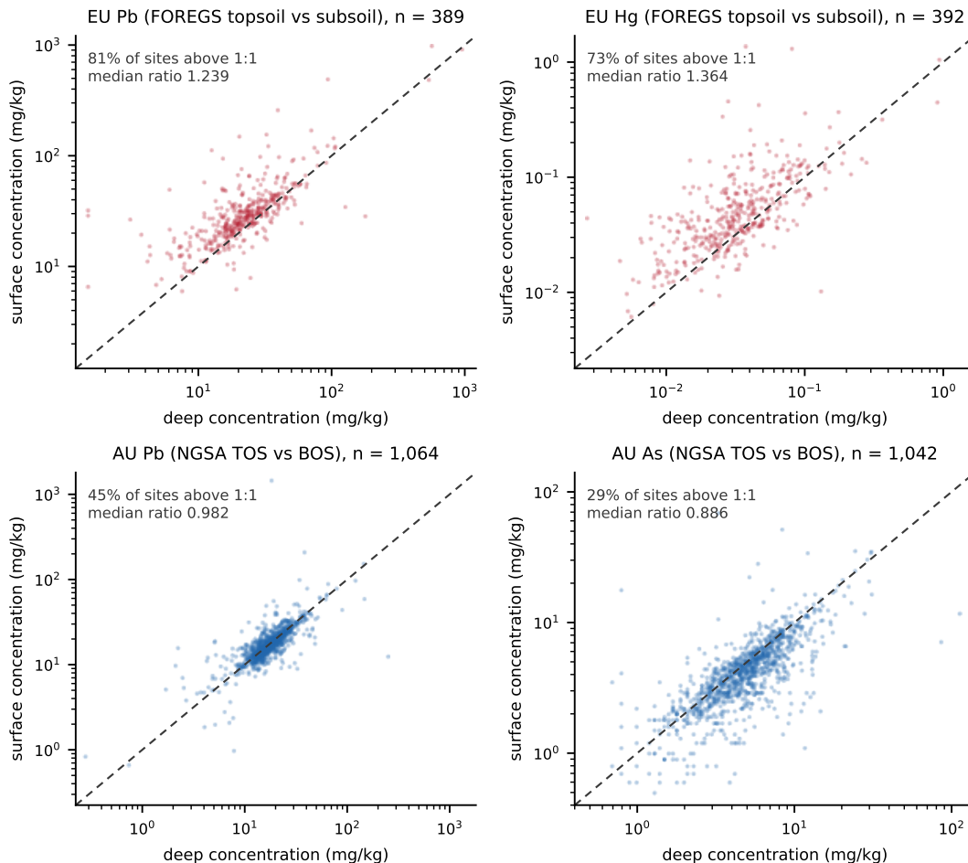
Figure 1: Raw site-paired concentrations (log-log; dashed line 1:1). Top row: FOREGS Europe — topsoil sits systematically above subsoil for Pb and Hg. Bottom row: NGSA Australia — Top Outlet Sediment straddles the 1:1 line for Pb and falls below it for As. Annotations give the share of sites above the 1:1 line and the median ratio; methods per panel as in Table 1.
