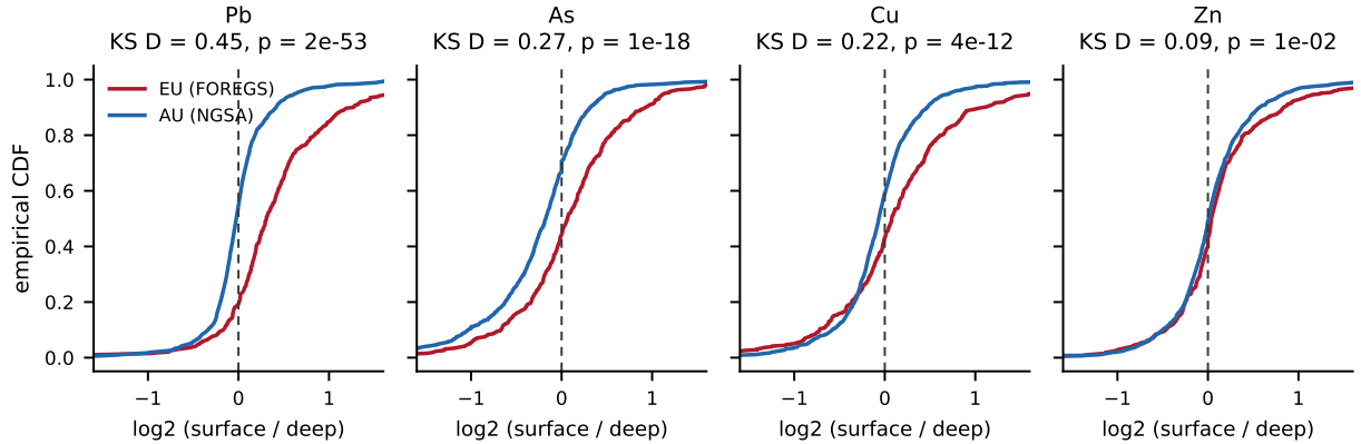
Figure 2: ECDFs of per-site \log_2 (surface/deep) ratios: Europe (FOREGS, red) versus Australia (NGSA, blue) for the four elements paired on both continents. Dashed line: no enrichment. Panel titles give the two-sample KS statistic and p -value.
