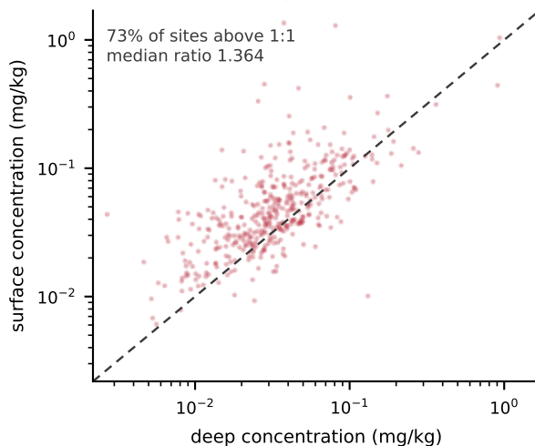
AU As (NGSA TOS vs BOS), n = 1,042
