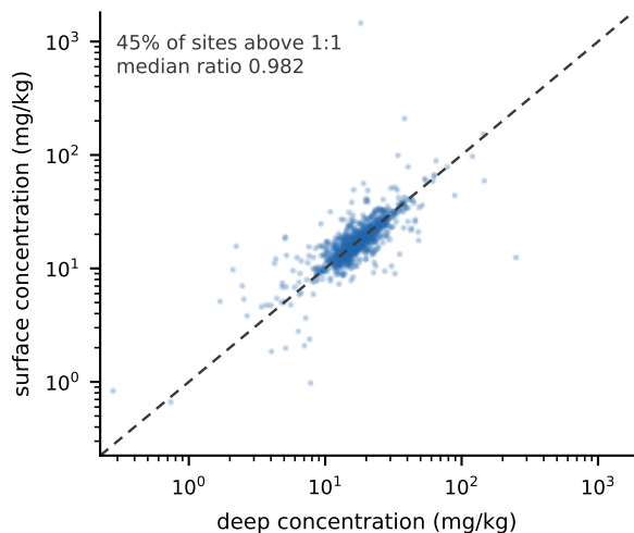
AU Pb (NGSA TOS vs BOS), n = 1,064
