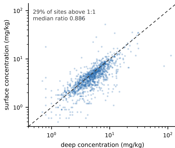
AU As (NGSA TOS vs BOS), n = 1,042
