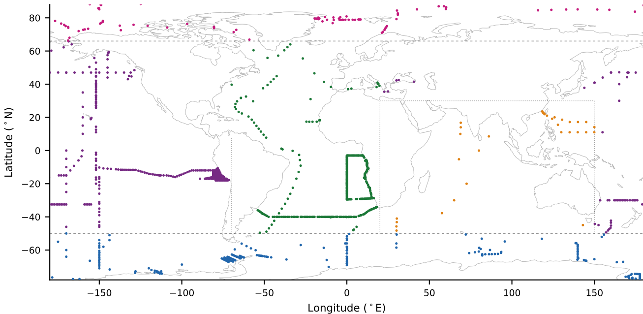
Harmonized GEOTRACES IDP2025 sampling positions (18,563 records, 1,005 positions)
