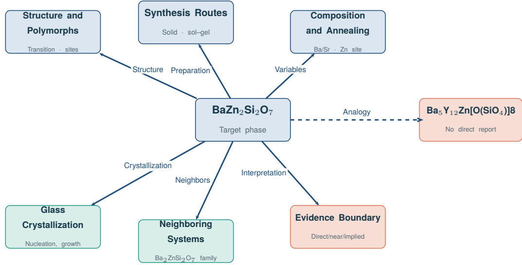
Figure 2. Taxonomy of \text{BaZn}_2\text{Si}_2\text{O}_7 synthesis and phase control. Solid branches carry direct experimental evidence for the target phase or experimental evidence from structurally related compounds; dashed nodes mark comparison targets for which no direct structural report exists.
