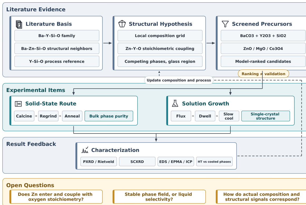
Figure 1. Research roadmap. The Ba–Y–Si–O, Ba–Zn–Si–O, and Y–Si–O systems are used first to establish structural relationships, competing phases, and process boundaries; phase-diagram and charge-balance analysis proposes candidate compositions, and the two-step inorganic retrosynthesis model supplies the precursor set; solid-state reaction and high-temperature solution growth probe the bulk phase region and the single-crystal structure, respectively, and the characterization results feed back into the next round of compositions and processes.
