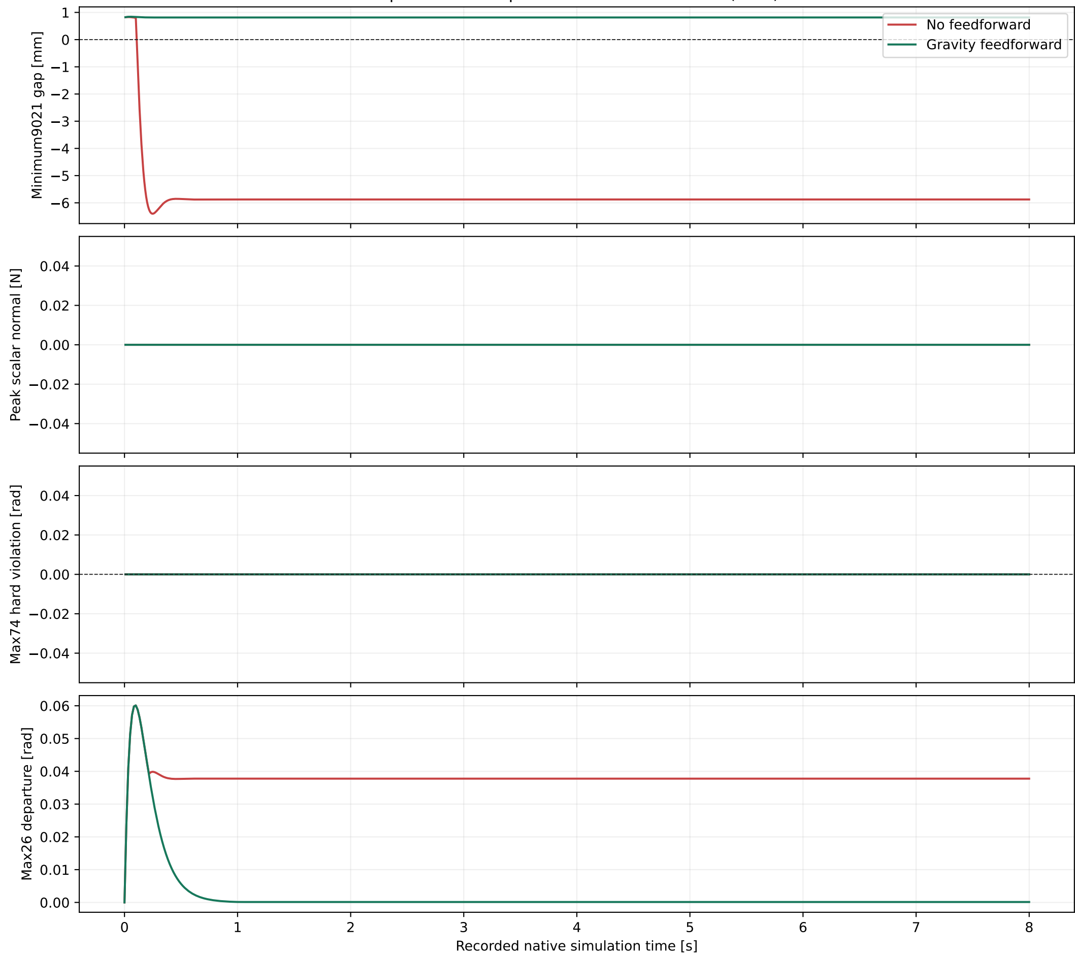
Input6447: held positions over 480 controls (~8 s)
