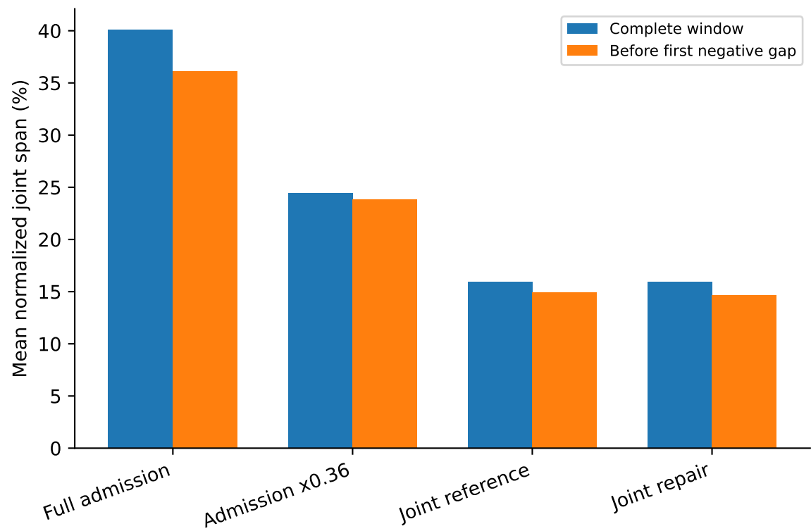
Motion retained
