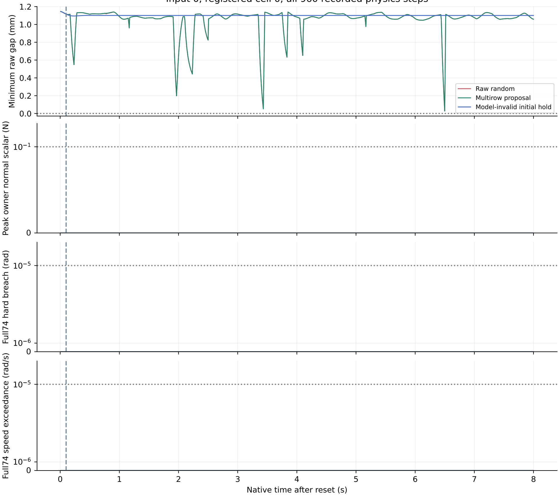
Input 0, registered cell 0; all 960 recorded physics steps
