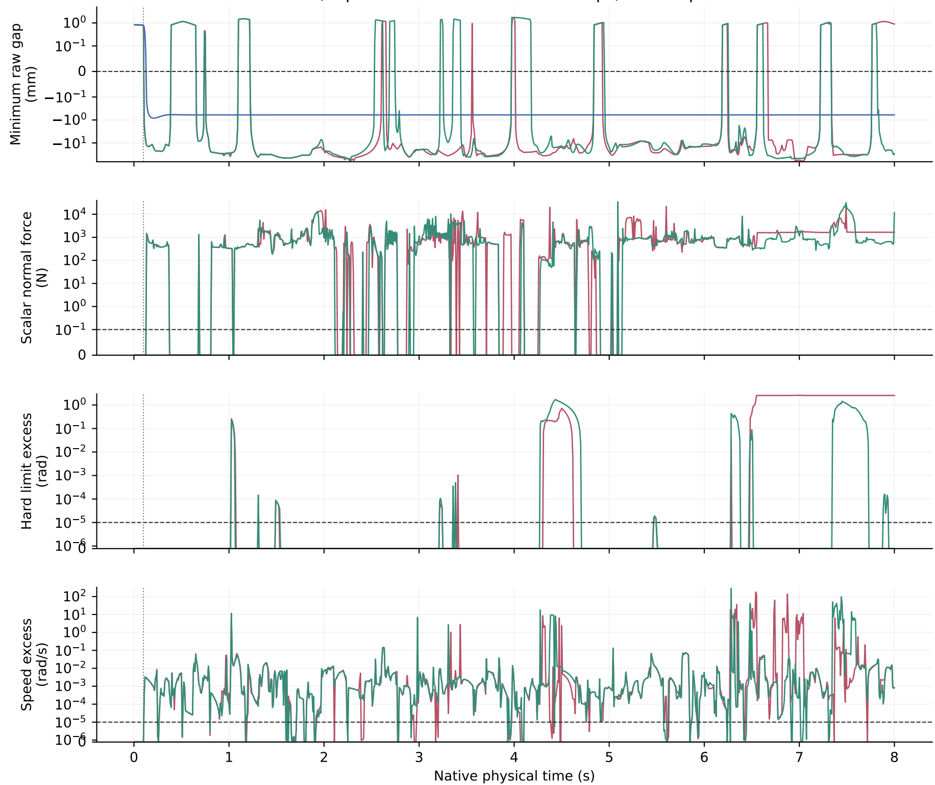
Cell 1, input 4168: all960 native substeps, no interpolation
