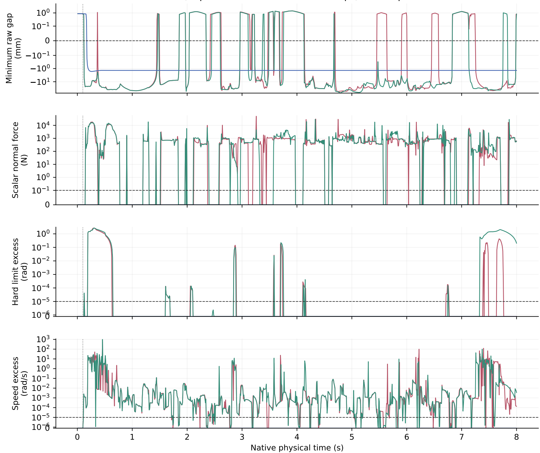
Cell 9, input 3254: all960 native substeps, no interpolation
