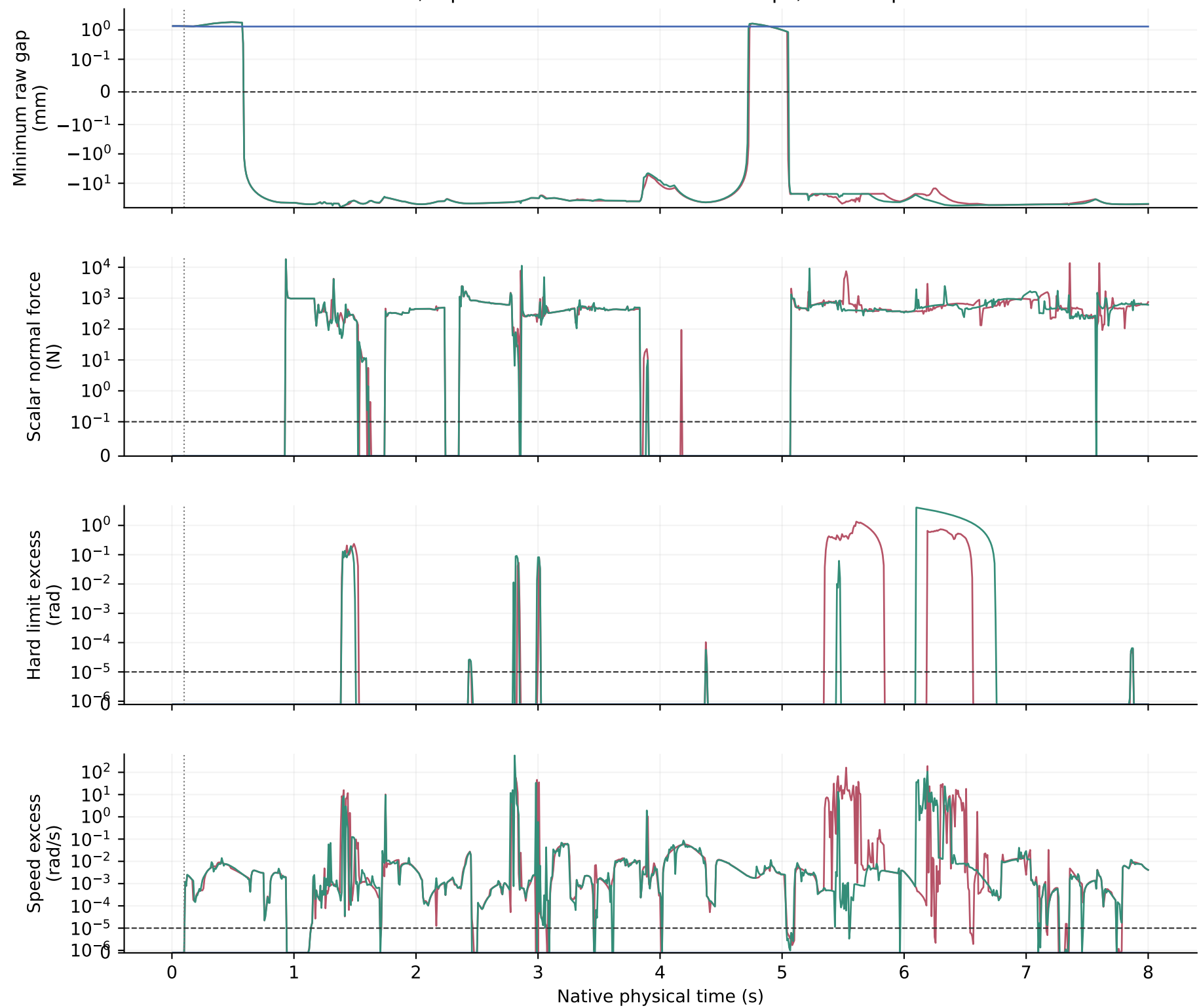
Cell 15, input 1212: all960 native substeps, no interpolation
