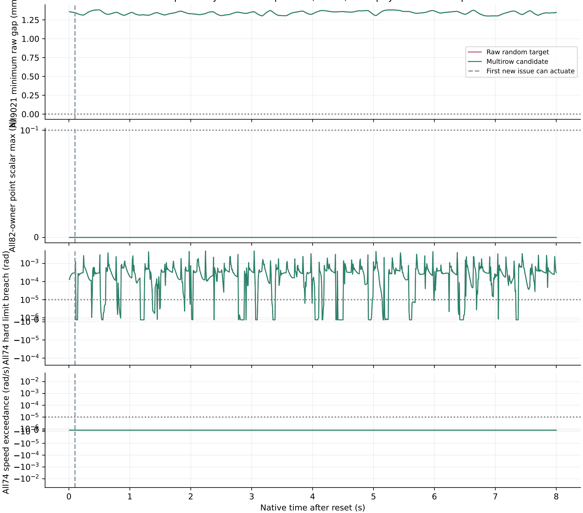
Prospectively selected input 112, cell 0; both physical microsteps
