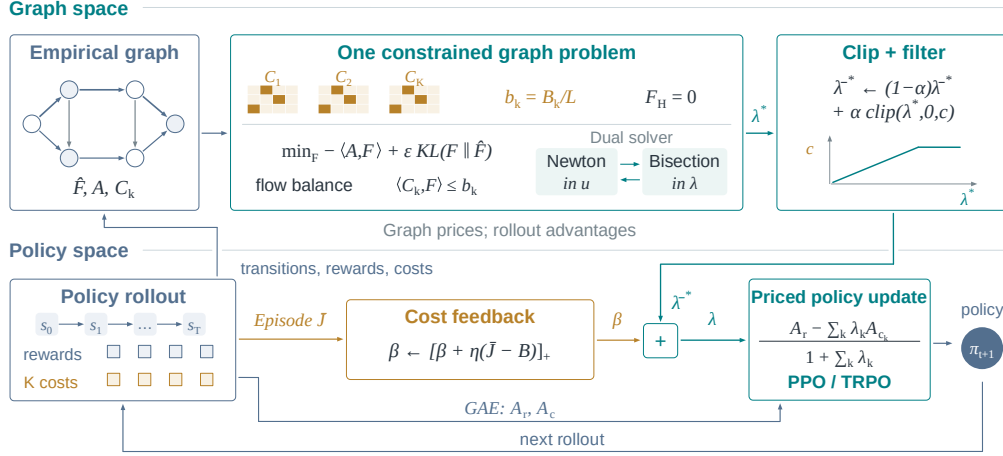
Figure 2: From constraints to the policy update. Rollouts supply an empirical graph, GAE advantages and episode-cost feedback. Graph budgets use b_k = B_k/L ; feedback uses B_k . Only the solved prices cross from the graph to the policy surrogate, after clipping and filtering. The next policy supplies the next rollout. Graph feasibility alone does not certify policy safety; the separate off-policy executor is not shown.
