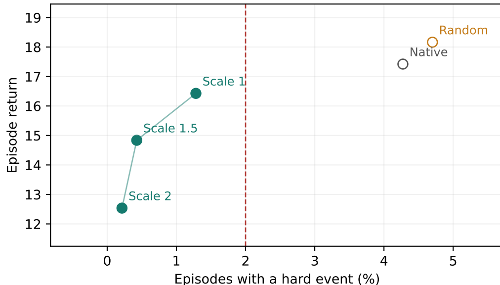
PointGoal2 / trained margin 0.9
