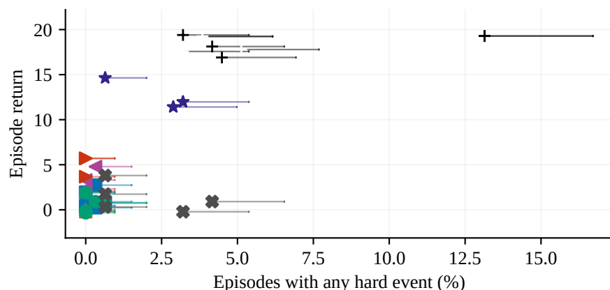
PointGoal2
