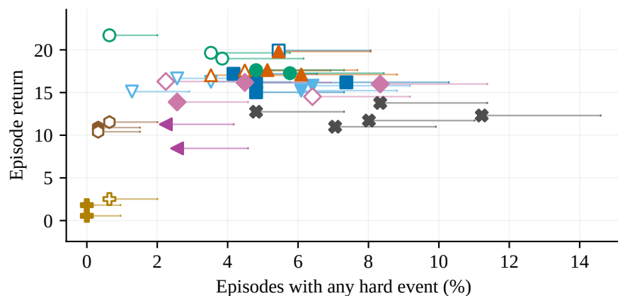
CarGoal2
