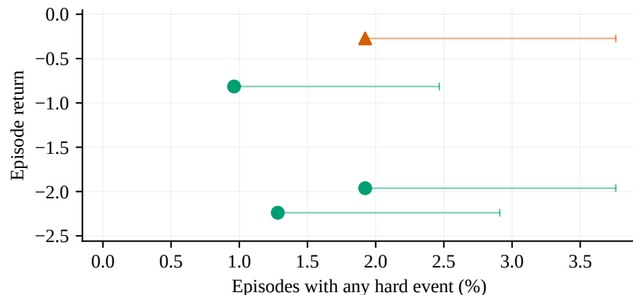
PointButton2
