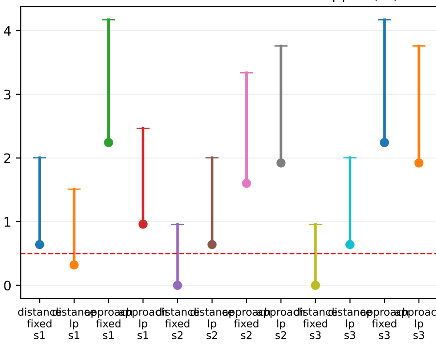
Hard-event rate & one-sided95% upper (%)
