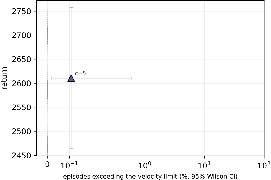
Walker2dVelocity
