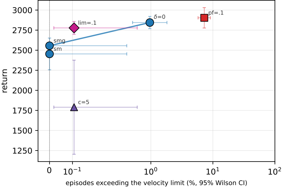
Walker2dVelocity
