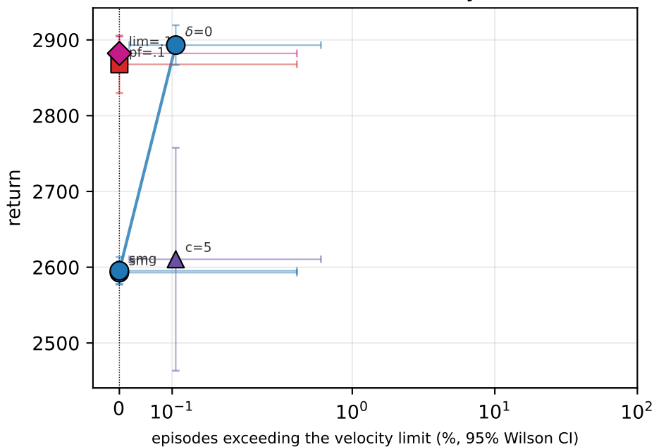
Walker2dVelocity
