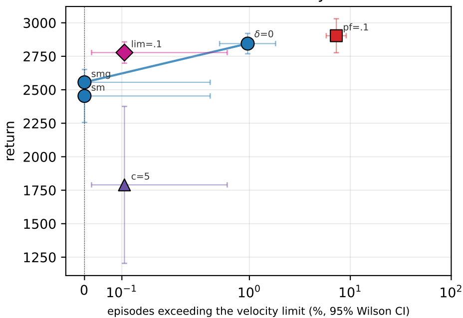
Walker2dVelocity
