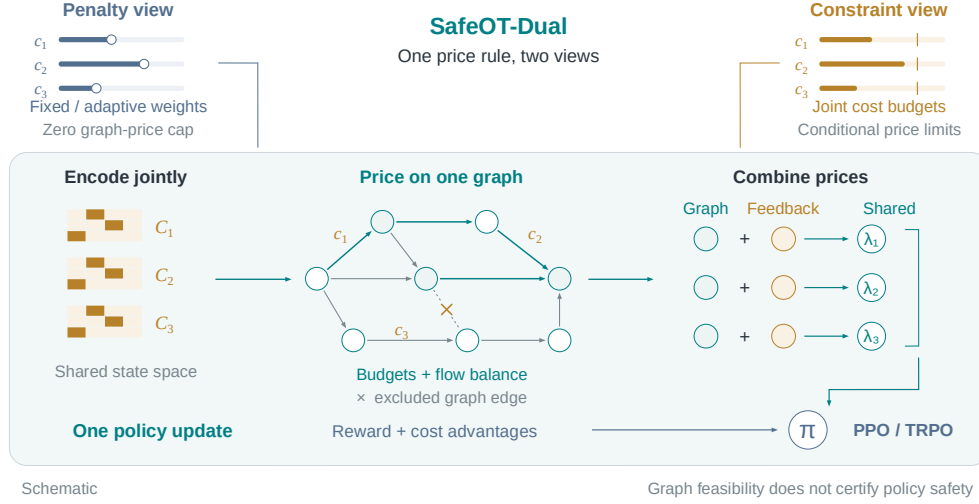
Figure 1: One safety-price interface. A clipped, filtered graph price is added to realized-cost feedback before pricing the policy advantages. At zero graph cap, fixed feedback gives a fixed penalty and adaptive feedback gives a Lagrangian rule. The graph LP and active-set limits require the assumptions in Section 3; they do not recover external algorithms such as CPO. Graphs are schematic.
