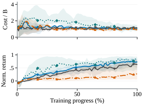
SafePO: 10 tasks, B = 25
