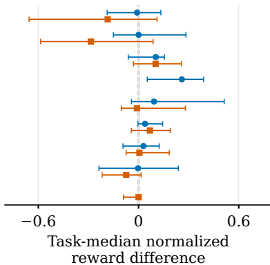
(b) Final-policy reward
