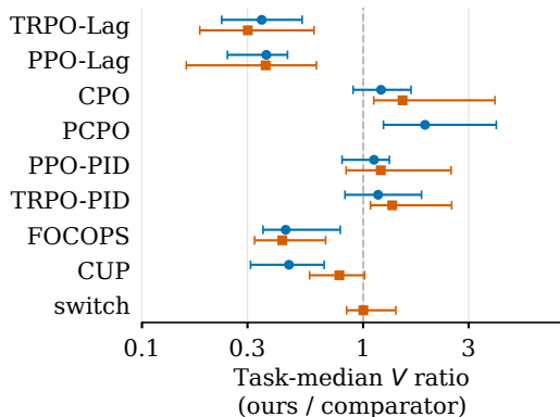
(a) Training violation
