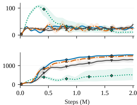
Hopper
