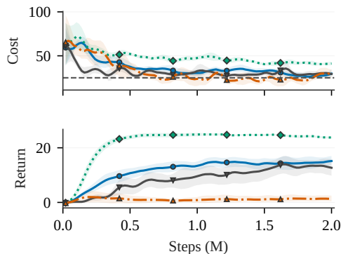
PointGoal1
