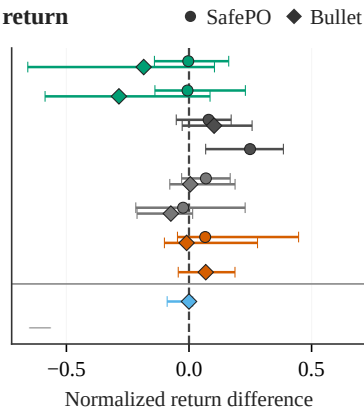
Hopper
