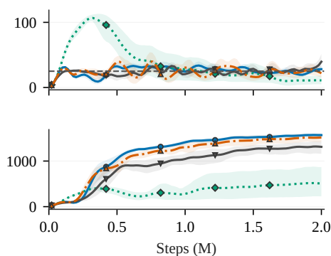
Hopper
