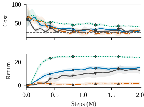
PointGoal1
