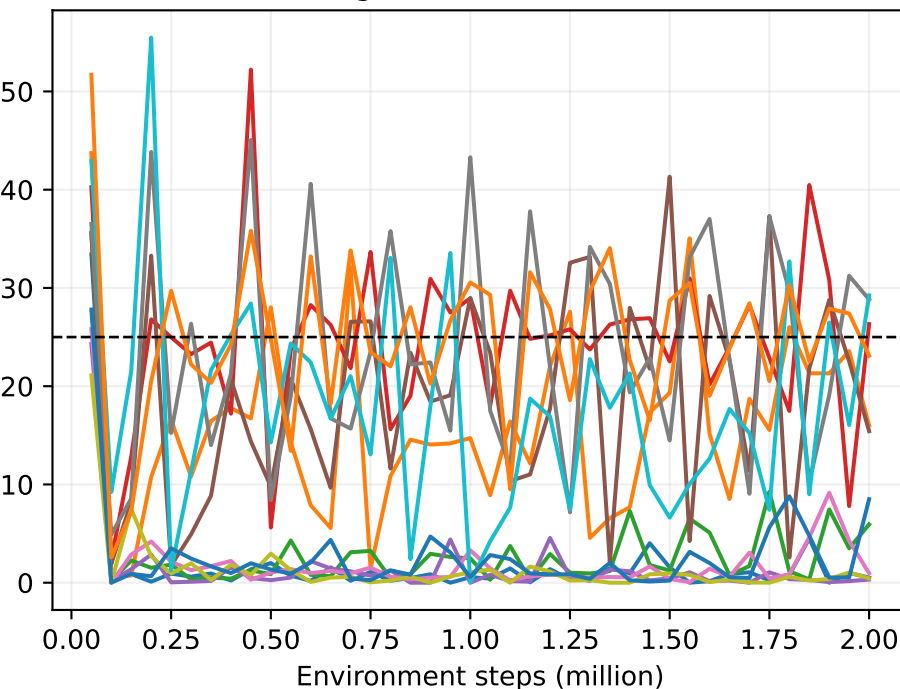
Final soft cost ± episode SE
