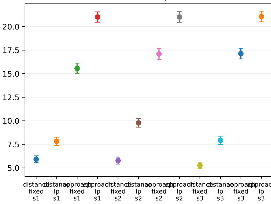
Final reward ± episode SE
