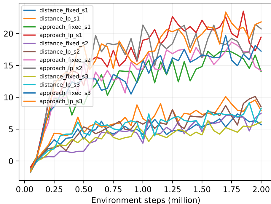
Final reward ± episode SE
