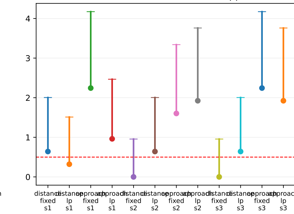
Hard-event rate & one-sided95% upper (%)
