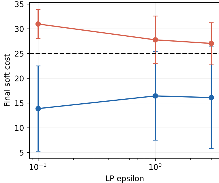
CG2: 18 completed policies / 5,616 episodes; mean \pm seed SD
