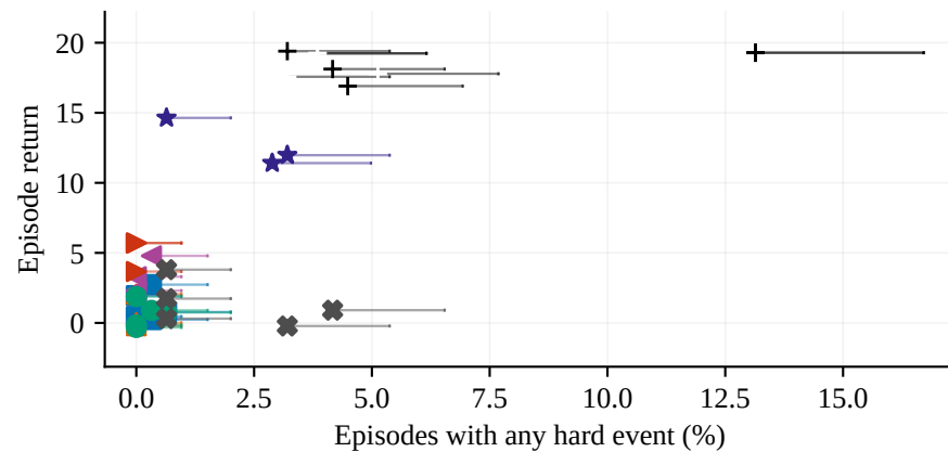
PointGoal2
