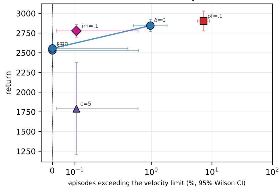
Walker2dVelocity
