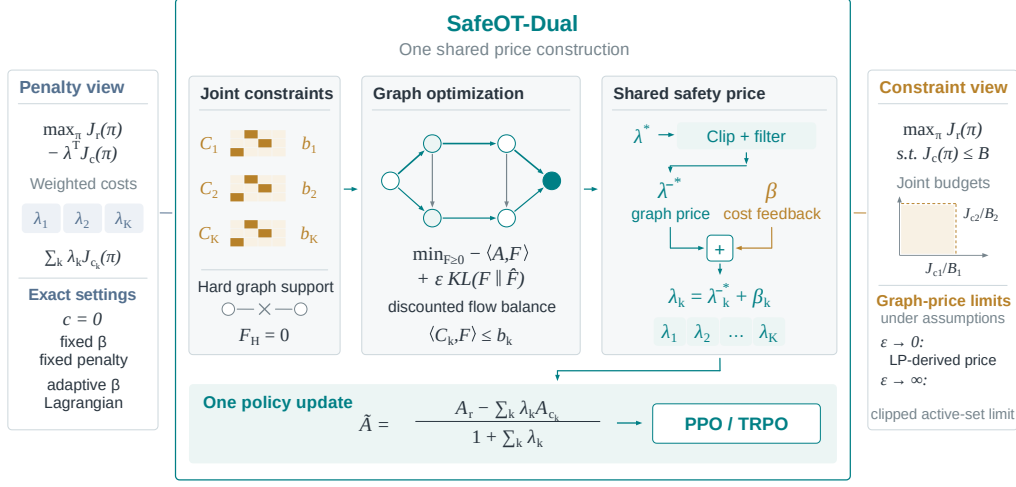
Figure 1: One safety-price interface. A clipped, filtered graph price is added to realized-cost feedback before pricing the policy advantages. At zero graph cap, fixed feedback gives a fixed penalty and adaptive feedback gives a Lagrangian rule. The graph LP and active-set limits require the assumptions in Section 3; they do not recover external algorithms such as CPO. Graphs are schematic.
