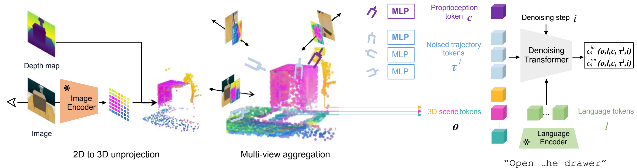
(a) 3D Diffuser Actor model architecture
