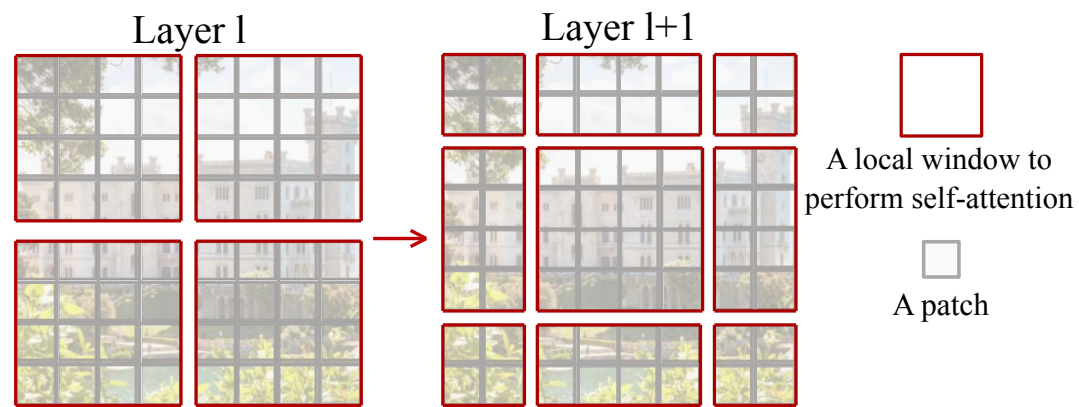
(b) Shifted Window
