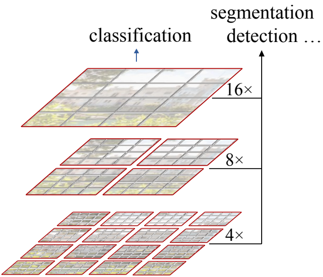
(a) Swin Transformer
