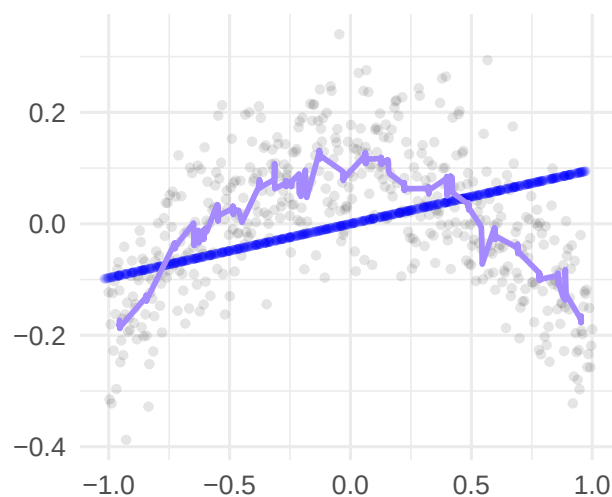
ManLe
