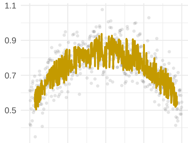
ManLe
