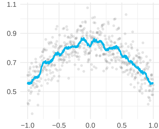
Nadaraya-Watson-Knn
