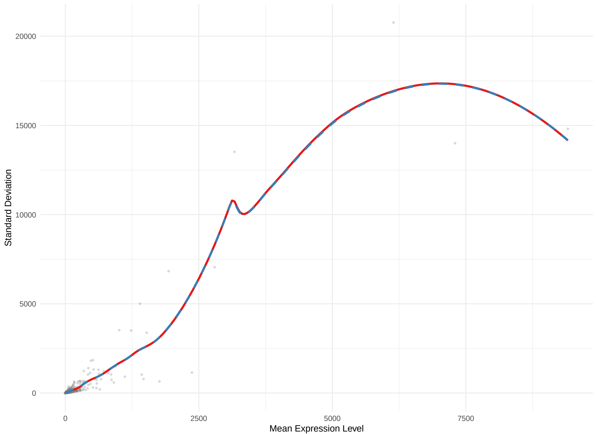
Gene Expression: Mean vs Standard Deviation LOESS smoothing reveals heteroscedasticity pattern
