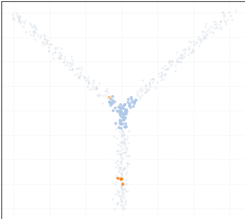
alpha_MAD = 0.25 [3 Clusters]
