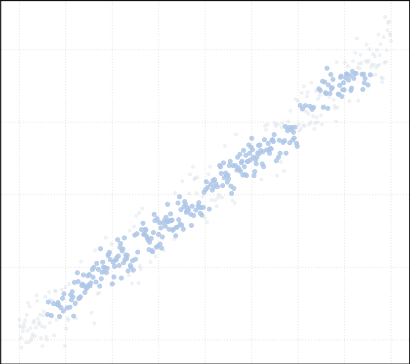
alpha_MAD = 0.75 [1 Clusters]
