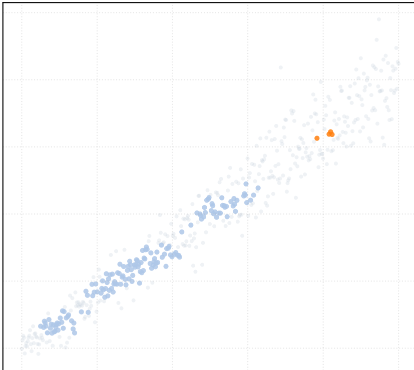
alpha_MAD = 0.25 [2 Clusters]
