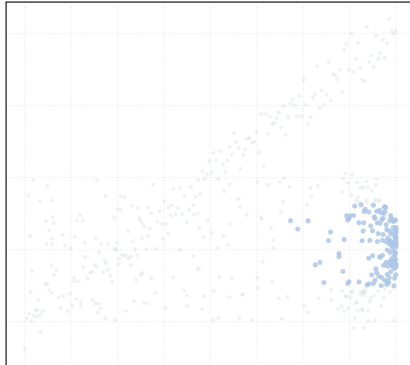
alpha_MAD = 0.75 [1 Clusters]
