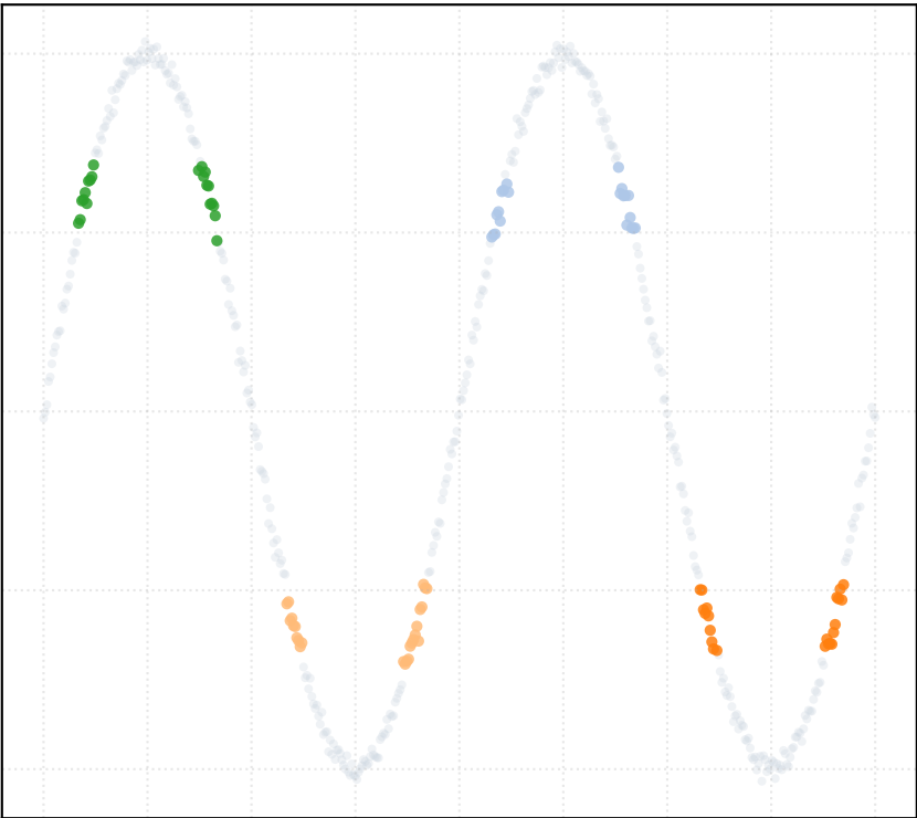
alpha_MAD = 0.25 [4 Clusters]
