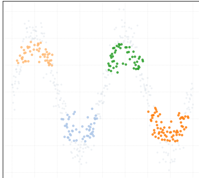
alpha_MAD = 0.75 [4 Clusters]
