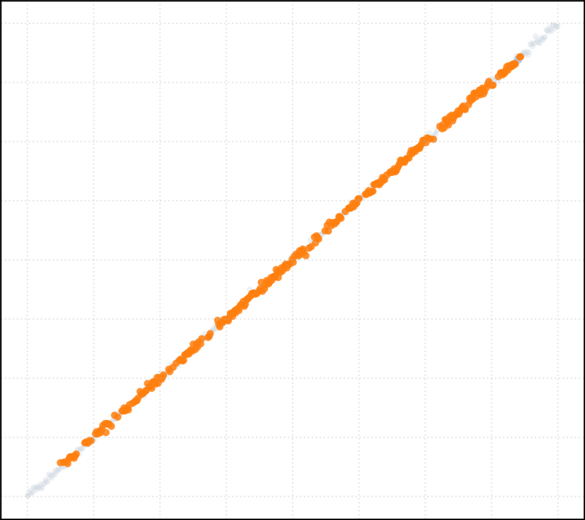
alpha_MAD = 1.0 [2 Clusters]
