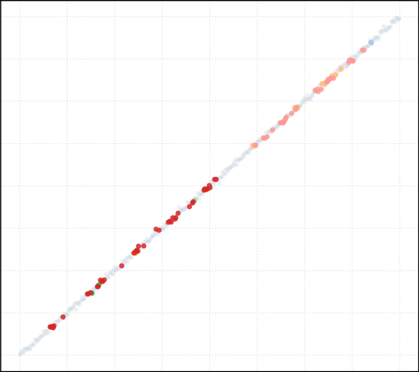
alpha_MAD = 0.75 [7 Clusters]
