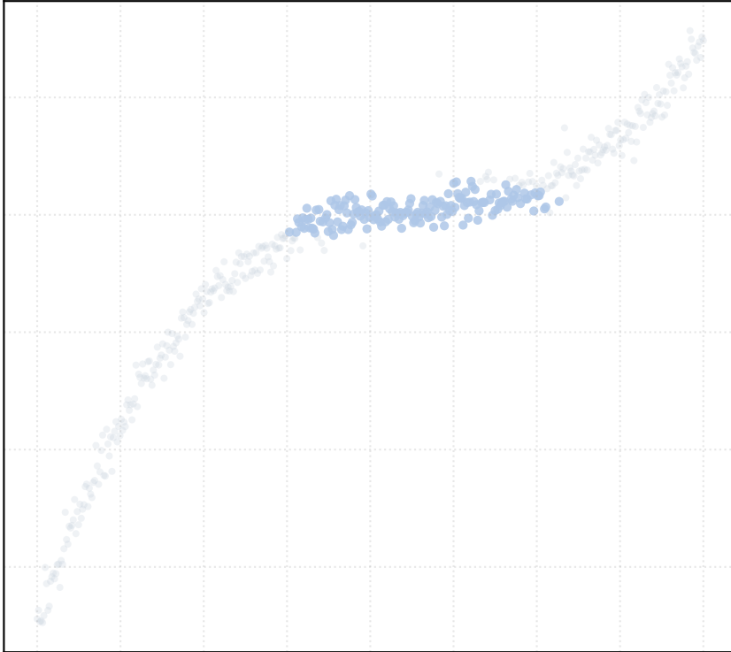
alpha_MAD = 0.75 [1 Clusters]
