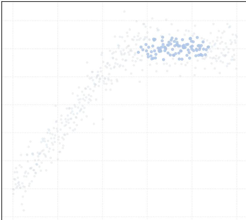
alpha_MAD = 0.25 [1 Clusters]
