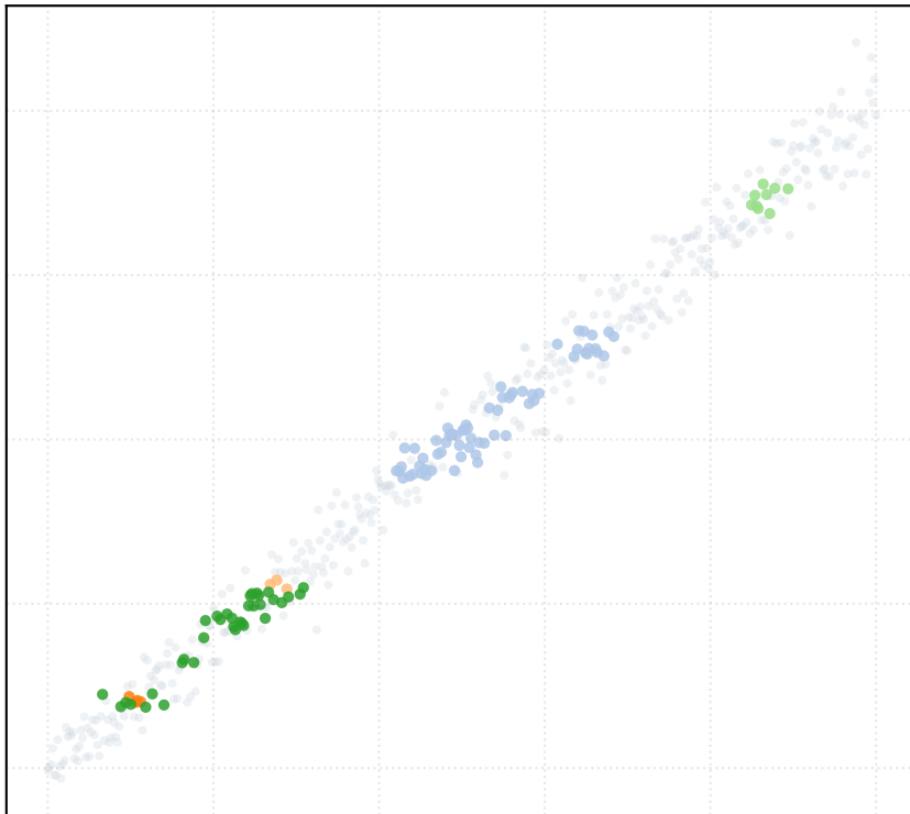
alpha_MAD = 0.25 [5 Clusters]
