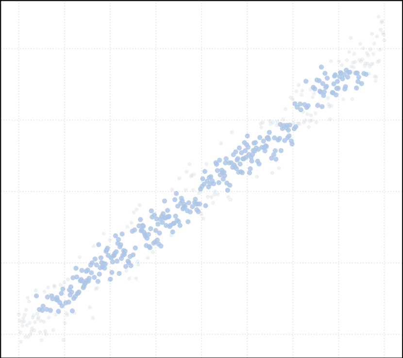
alpha_MAD = 1.0 [1 Clusters]
