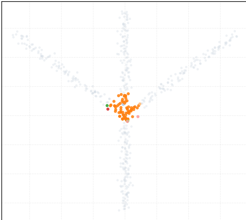
alpha_MAD = 0.25 [7 Clusters]
