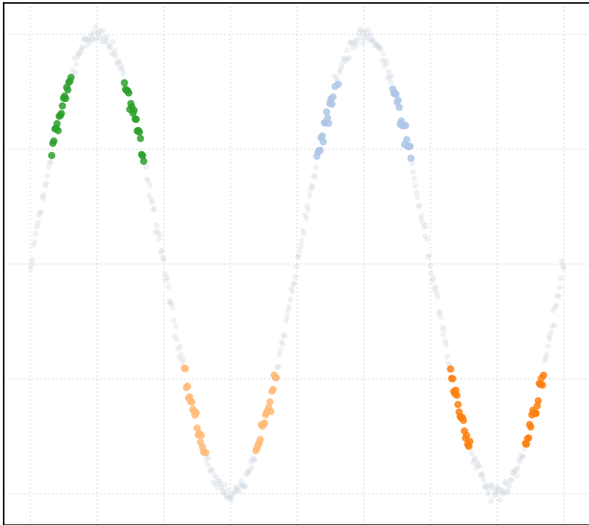
alpha_MAD = 1.0 [4 Clusters]
