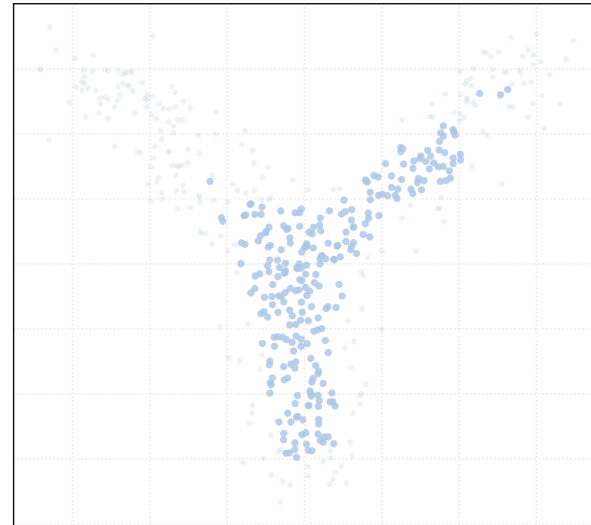
alpha_MAD = 1.0 [1 Clusters]
