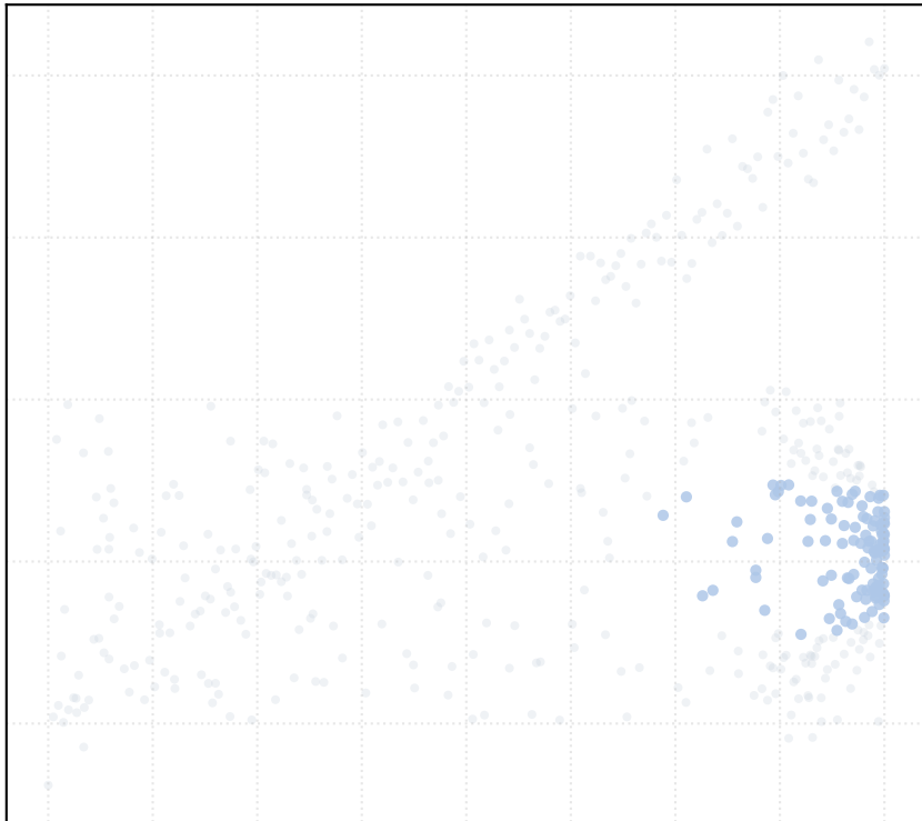
alpha_MAD = 0.25 [1 Clusters]
