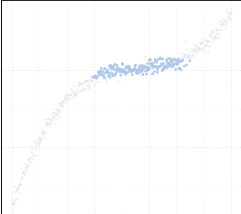
alpha_MAD = 1.0 [1 Clusters]
