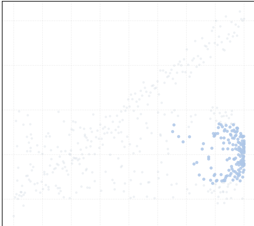
alpha_MAD = 1.0 [1 Clusters]
