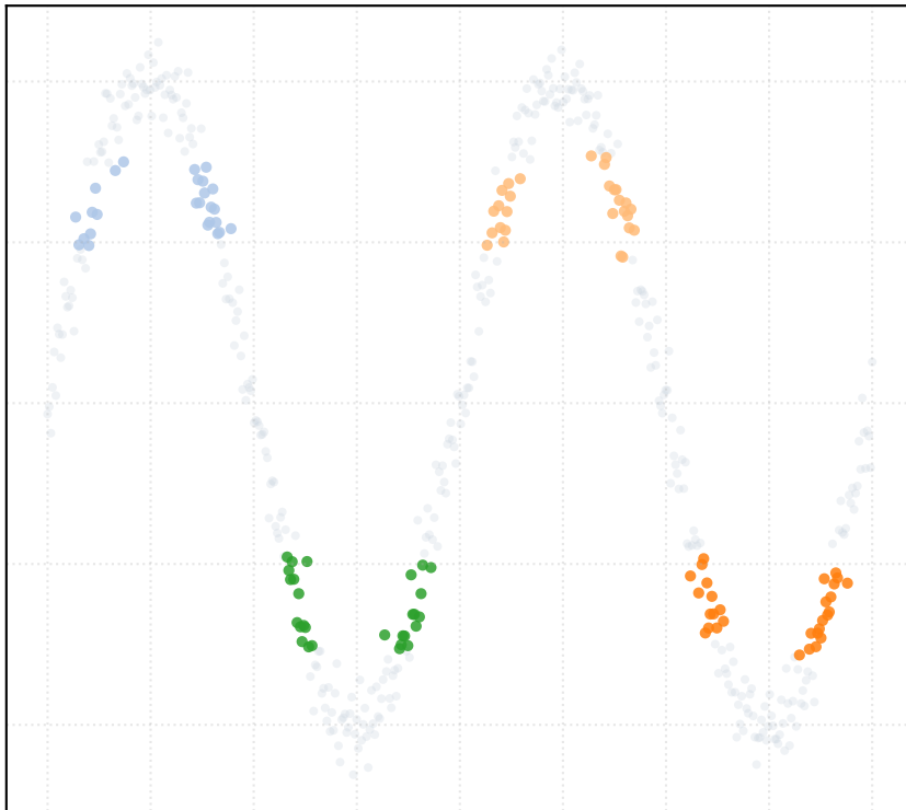
alpha_MAD = 0.25 [4 Clusters]
