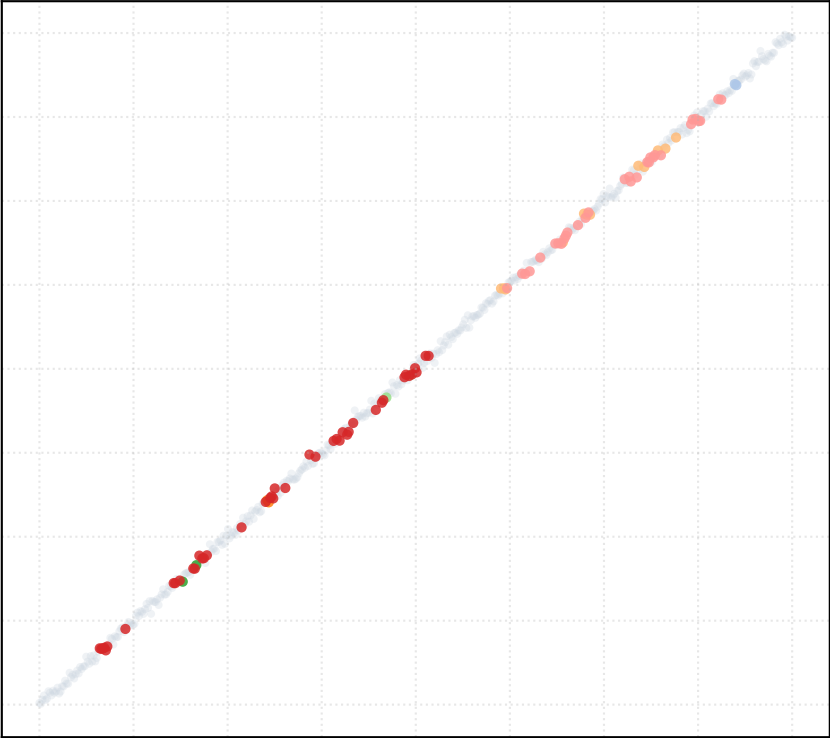
alpha_MAD = 0.25 [7 Clusters]
