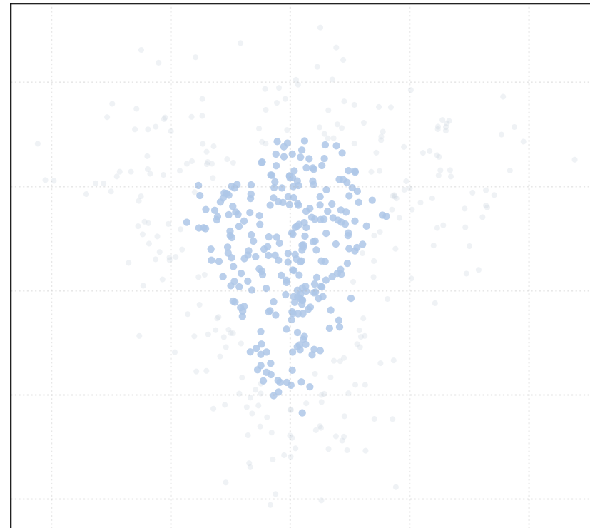
alpha_MAD = 1.0 [1 Clusters]
