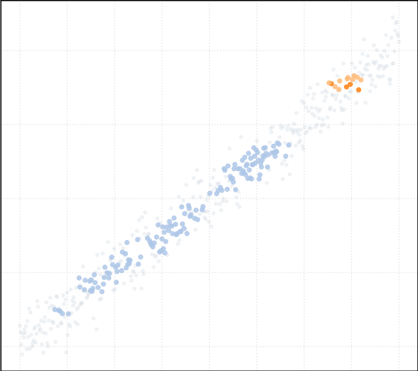
alpha_MAD = 0.25 [3 Clusters]
