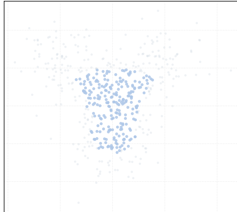
alpha_MAD = 0.75 [1 Clusters]
