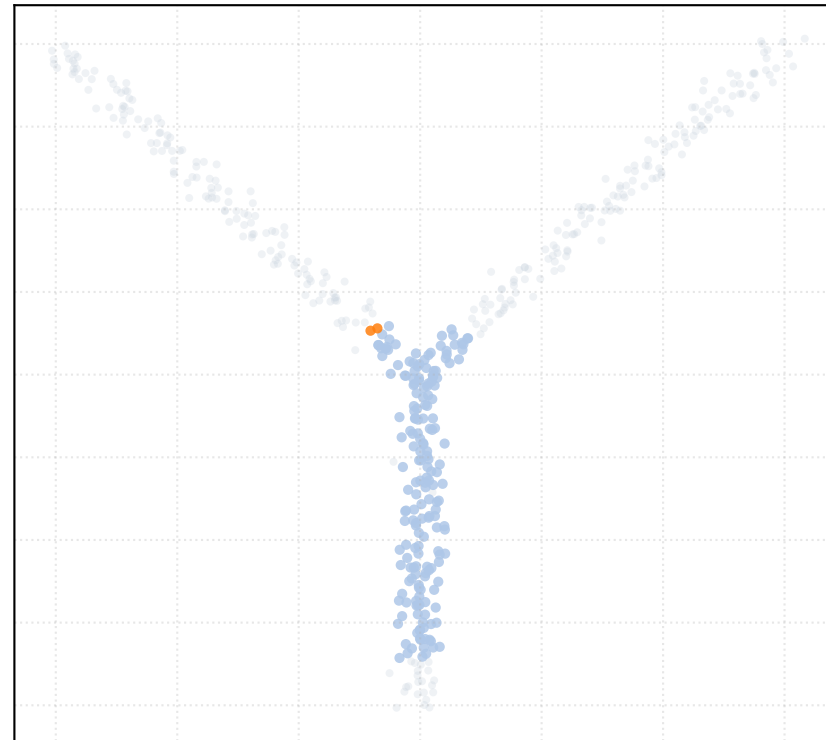
alpha_MAD = 0.75 [2 Clusters]
