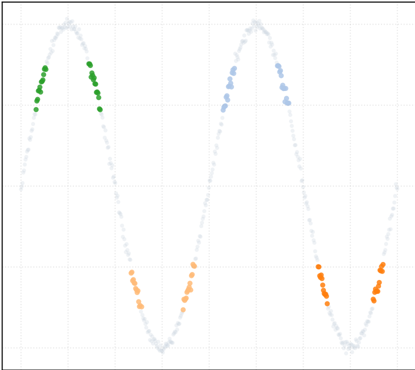
alpha_MAD = 0.75 [4 Clusters]
