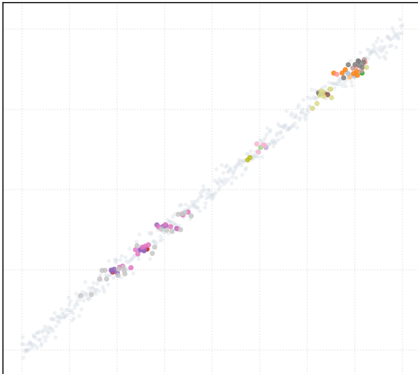
alpha_MAD = 0.25 [17 Clusters]
