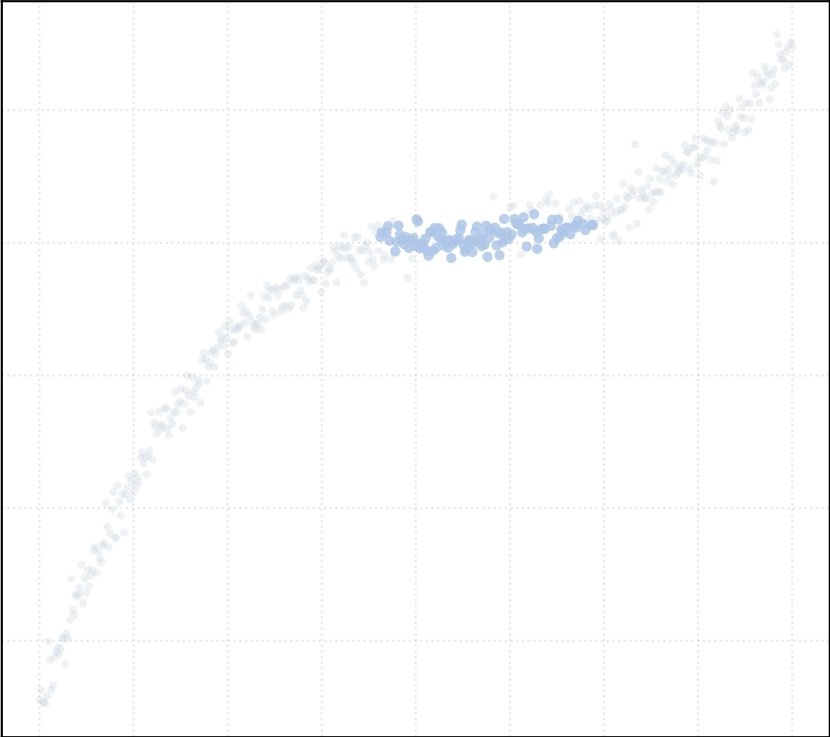
alpha_MAD = 0.25 [1 Clusters]
