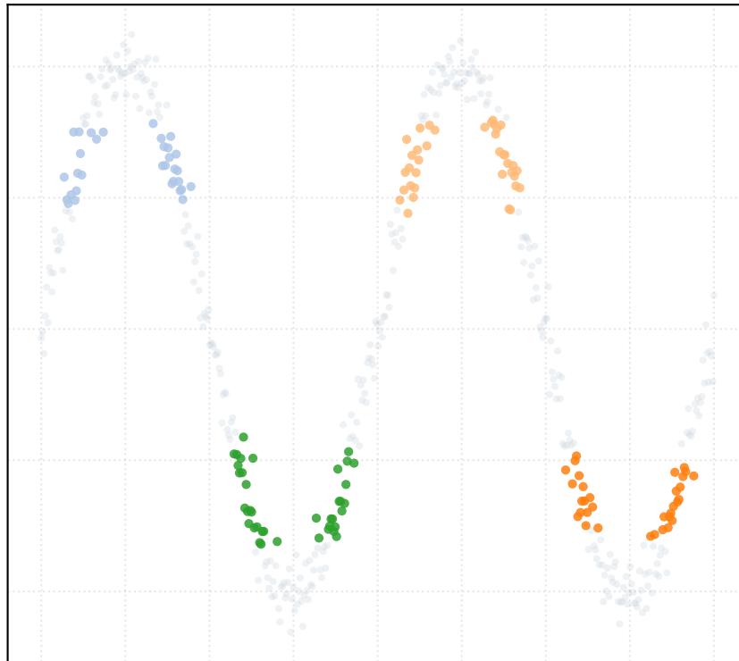
alpha_MAD = 0.5 (Default) [4 Clusters]
