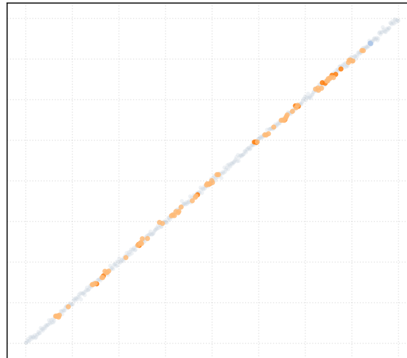
r = 3.0 [3 Clusters]
