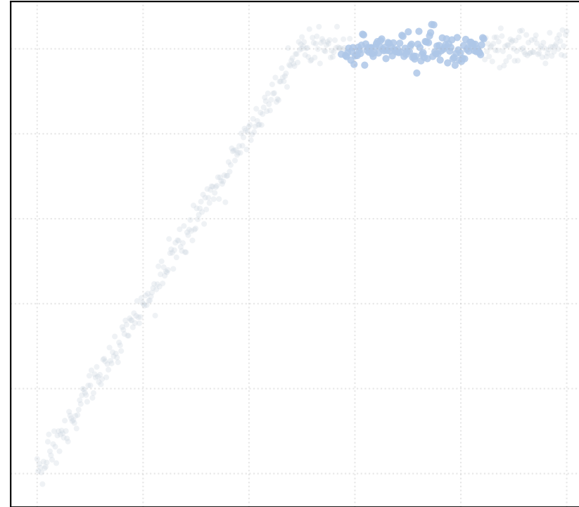
r = 3.5 [1 Clusters]
