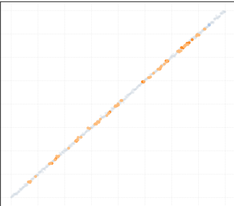
r = 2.0 [3 Clusters]
