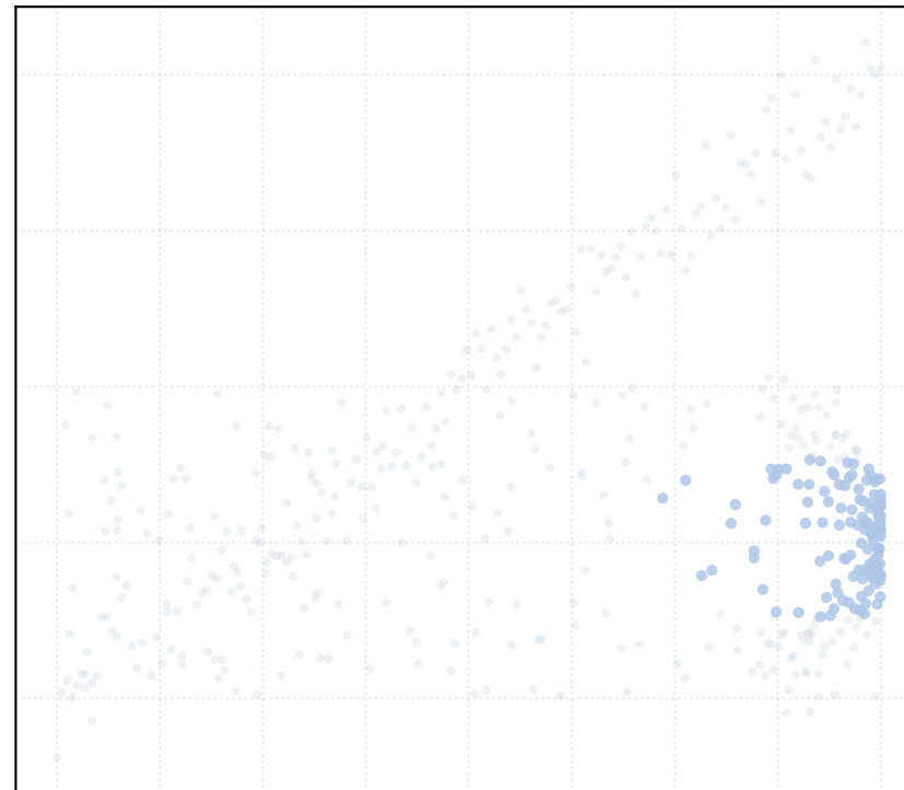
r = 3.0 [1 Clusters]
