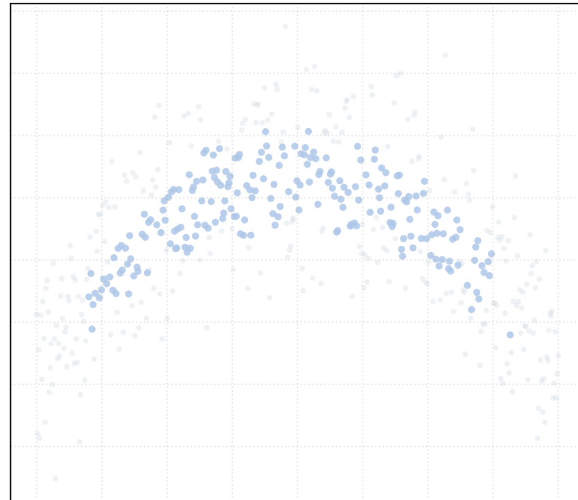
r = 3.5 [1 Clusters]
