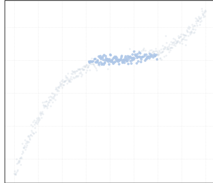
r = 3.5 [1 Clusters]
