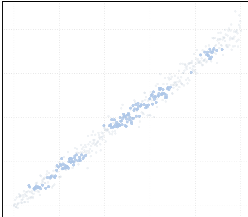
r = 2.5 [1 Clusters]
