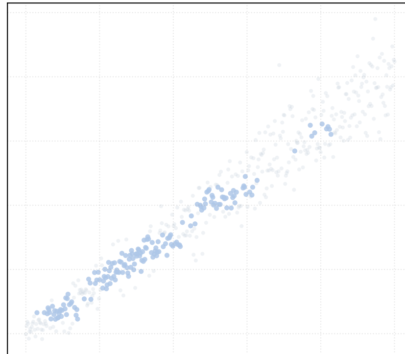
r = 3.5 [1 Clusters]
