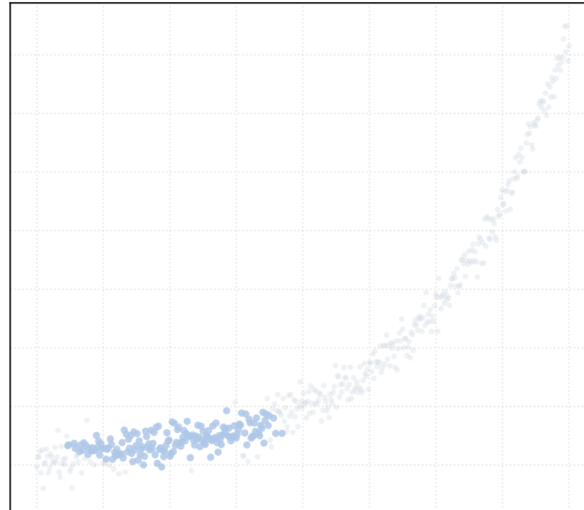
r = 3.0 [1 Clusters]
