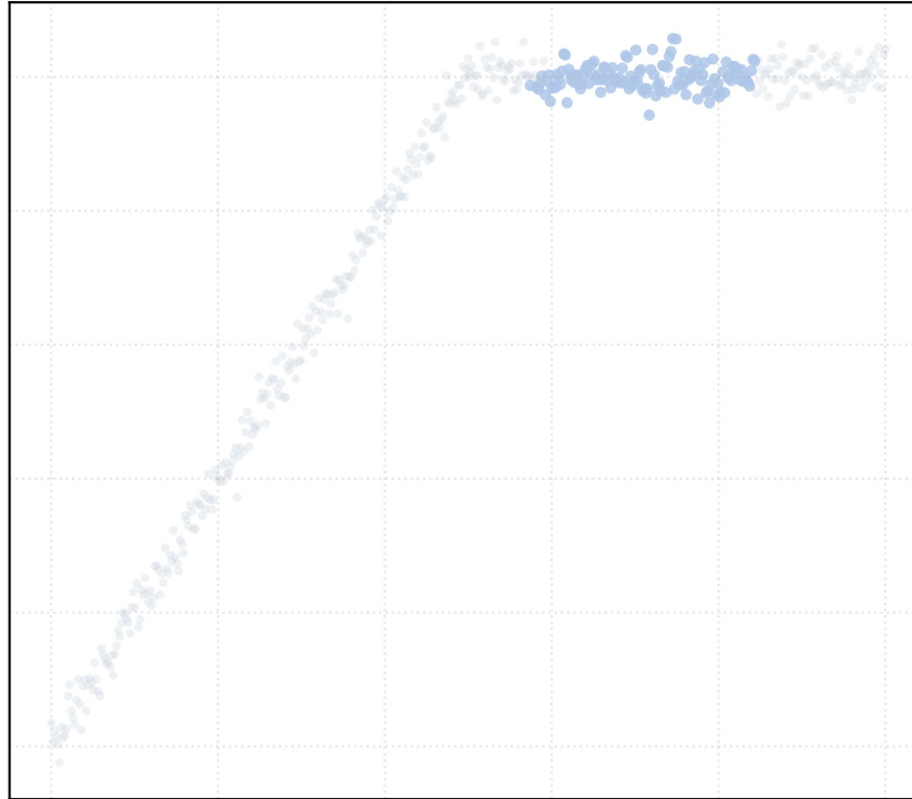
r = 2.5 [1 Clusters]
