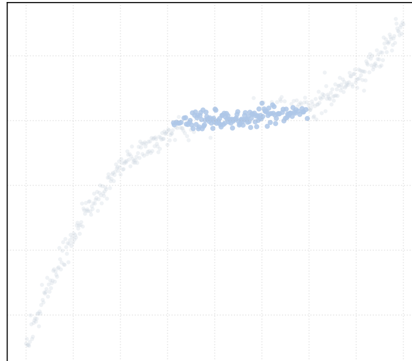
r = 3.0 [1 Clusters]
