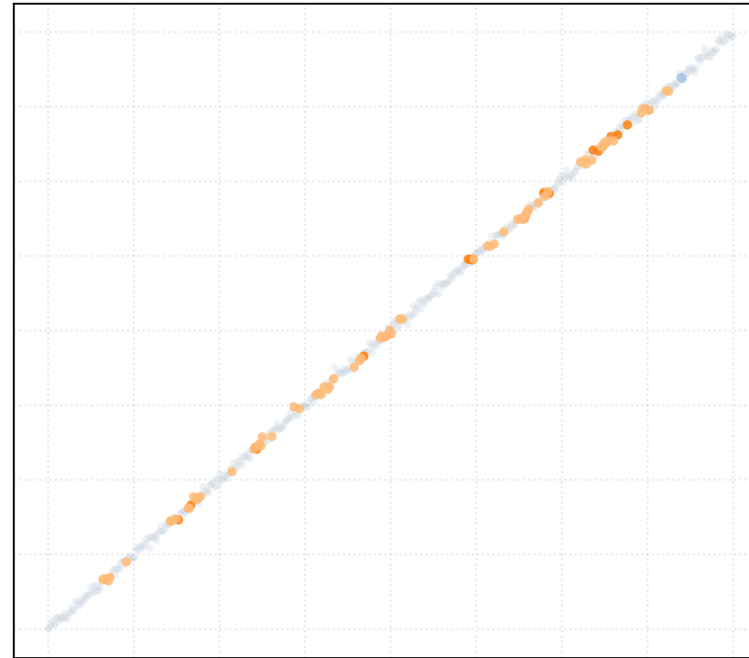
r = 3.5 [3 Clusters]
