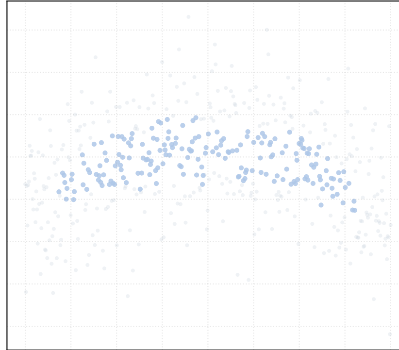
r = 3.0 [1 Clusters]
