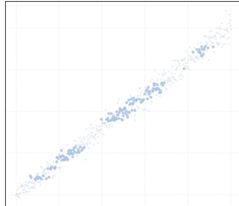
r = 3.5 [1 Clusters]
