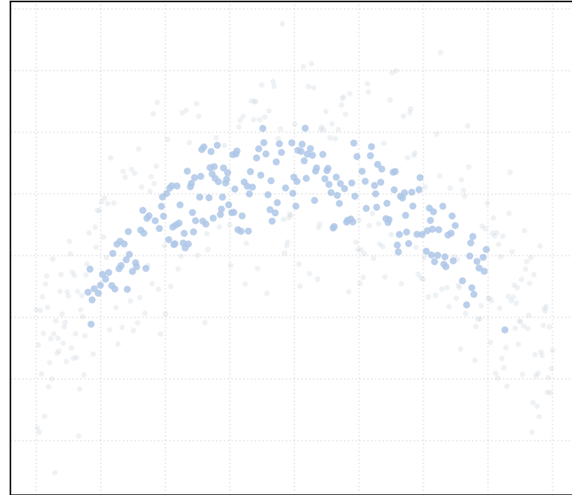
r = 3.5 [1 Clusters]
