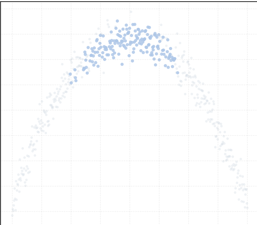
r = 2.0 [1 Clusters]
