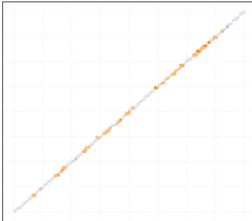
r = 2.5 [3 Clusters]
