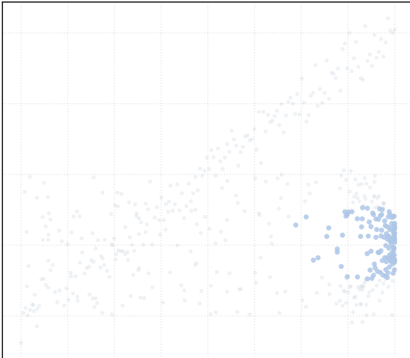
r = 2.0 [1 Clusters]
