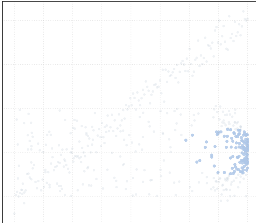
r = 2.5 [1 Clusters]
