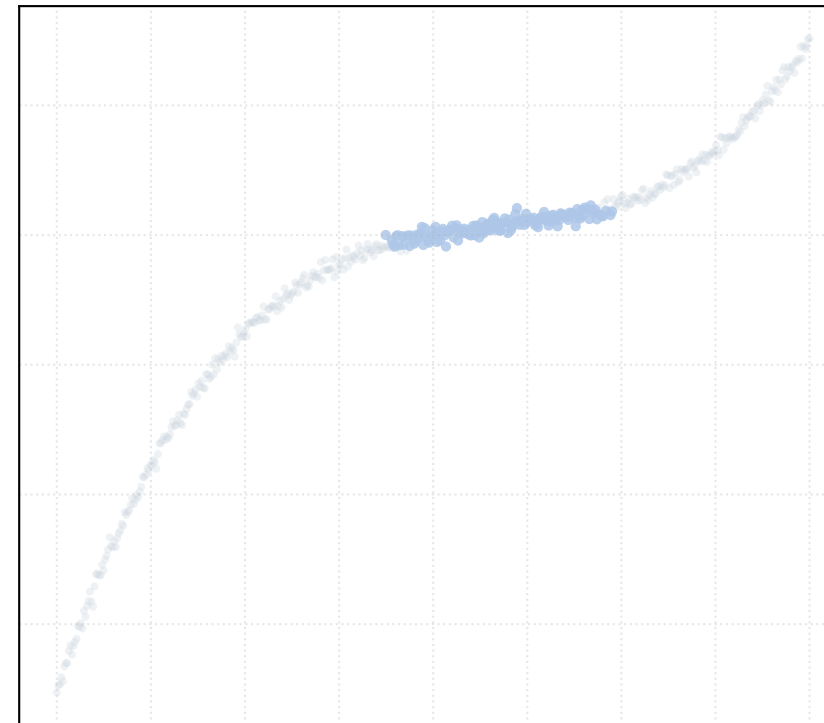
r = 3.5 [1 Clusters]
