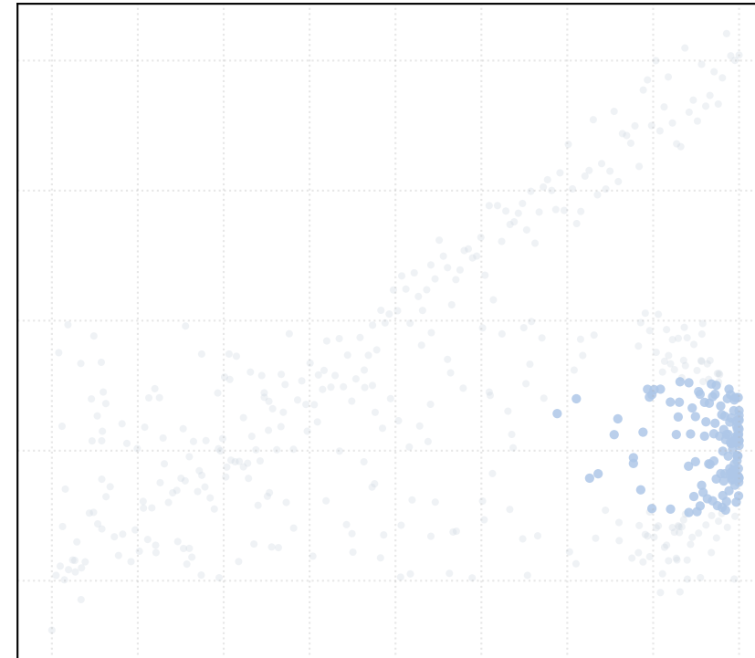
r = 3.5 [1 Clusters]
