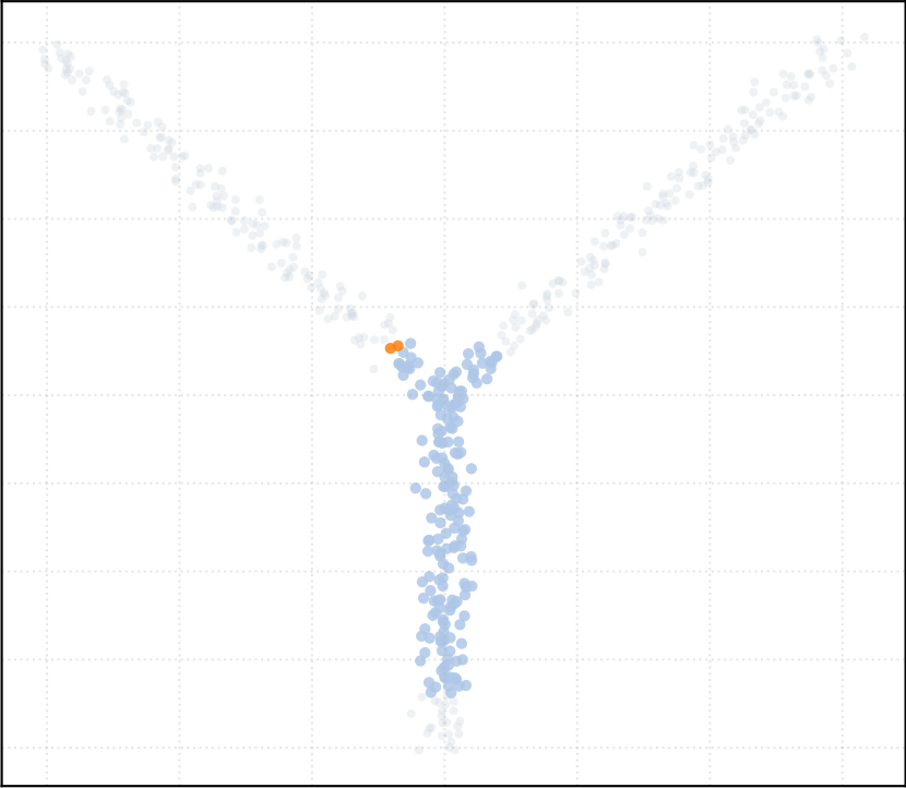
t_percentile = 0.3 [2 Clusters]
