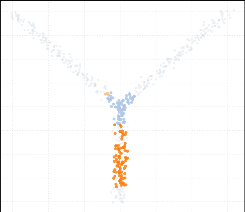
t_percentile = 0.4 [7 Clusters]
