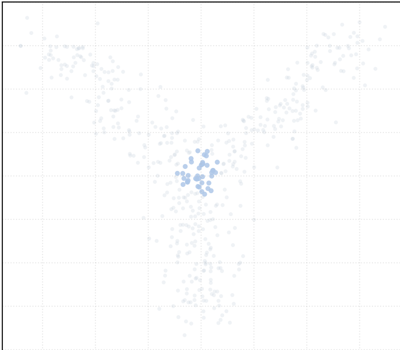
t_percentile = 0.25 [1 Clusters]
