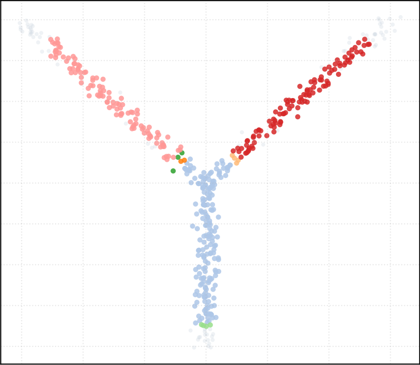
t_percentile = 0.4 [7 Clusters]
