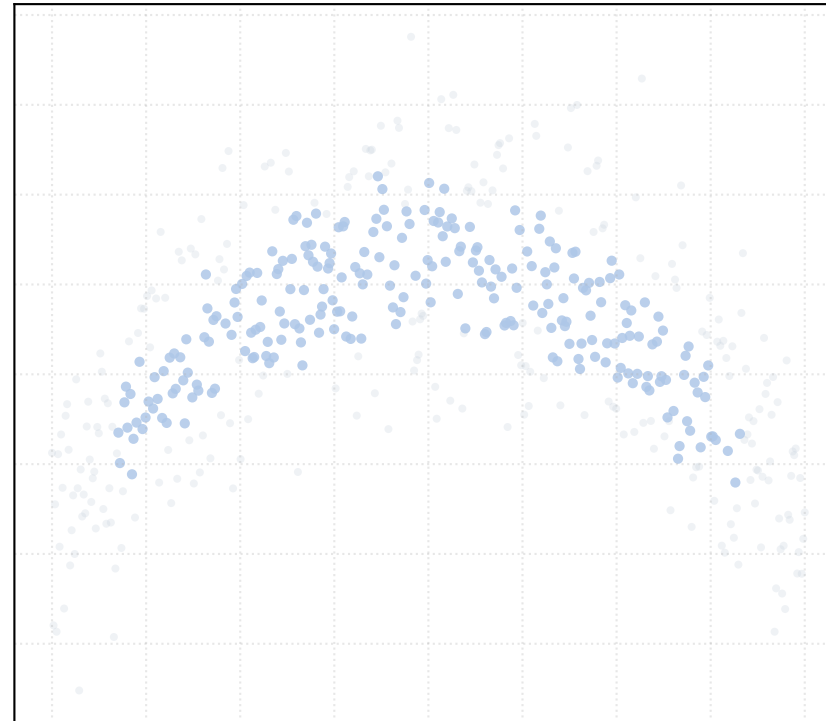
t_percentile = 0.4 [1 Clusters]
