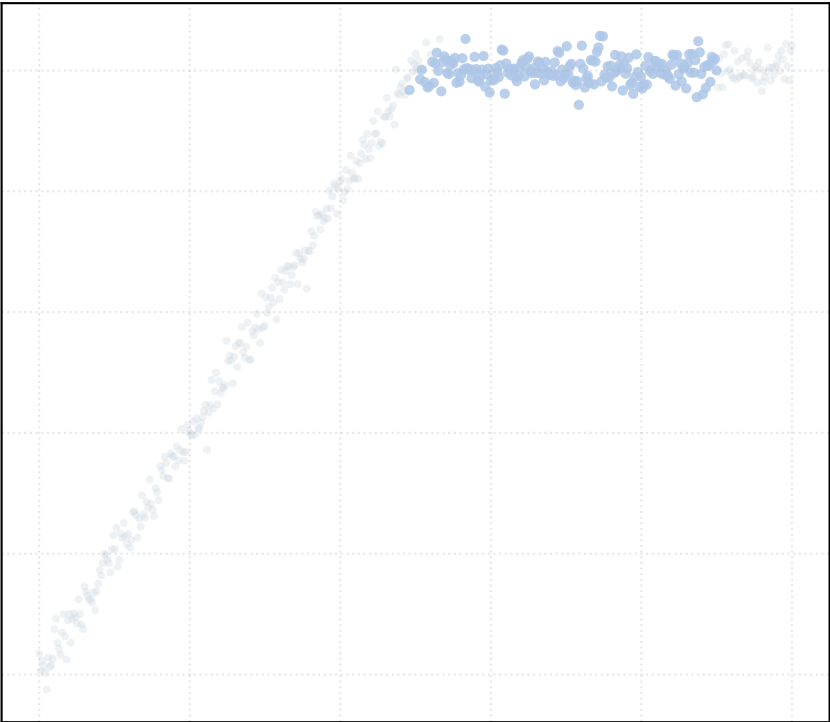
t_percentile = 0.3 [1 Clusters]
