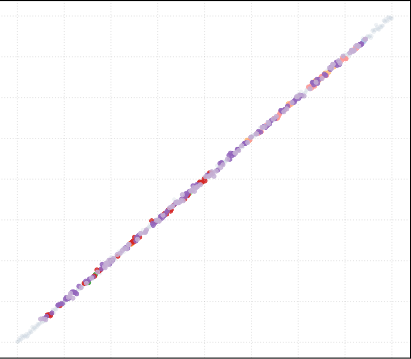
t_percentile = 0.5 [9 Clusters]
