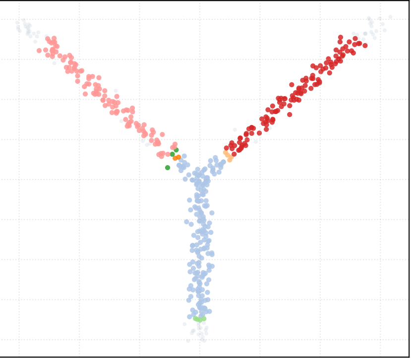
t_percentile = 0.5 [7 Clusters]
