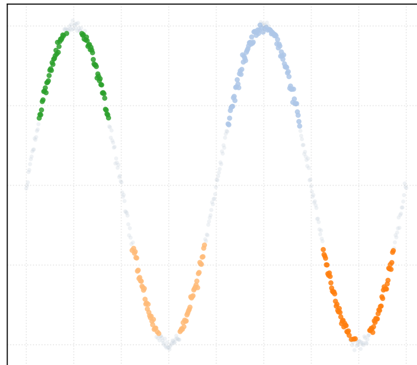
t_percentile = 0.4 [4 Clusters]
