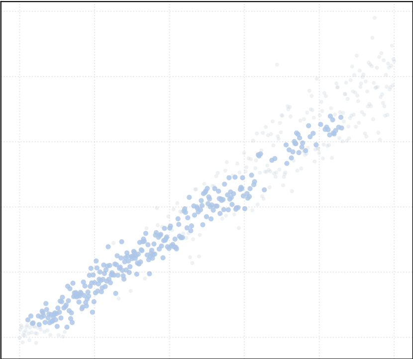
t_percentile = 0.25 [1 Clusters]
