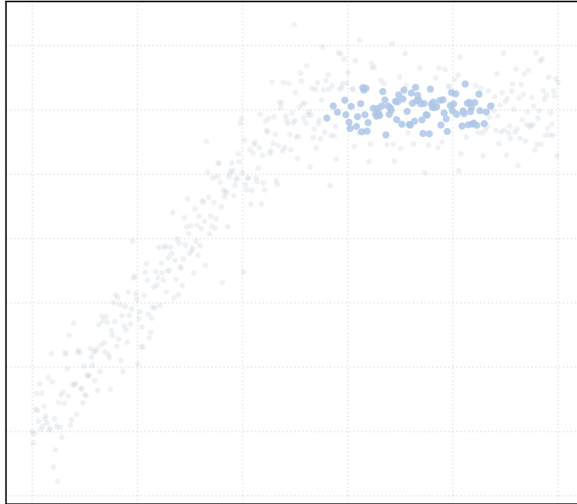
t_percentile = 0.3 [1 Clusters]
