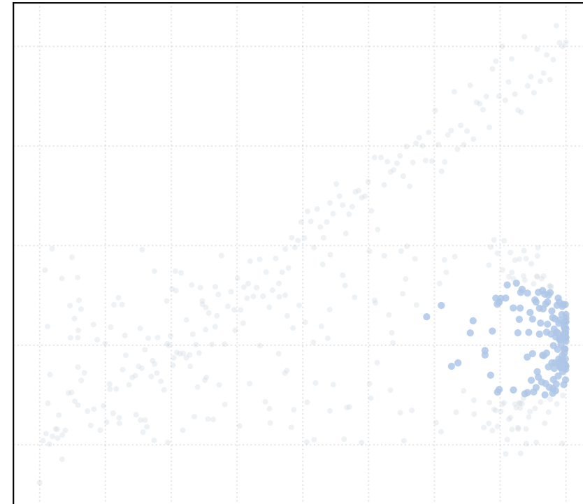
t_percentile = 0.5 [1 Clusters]
