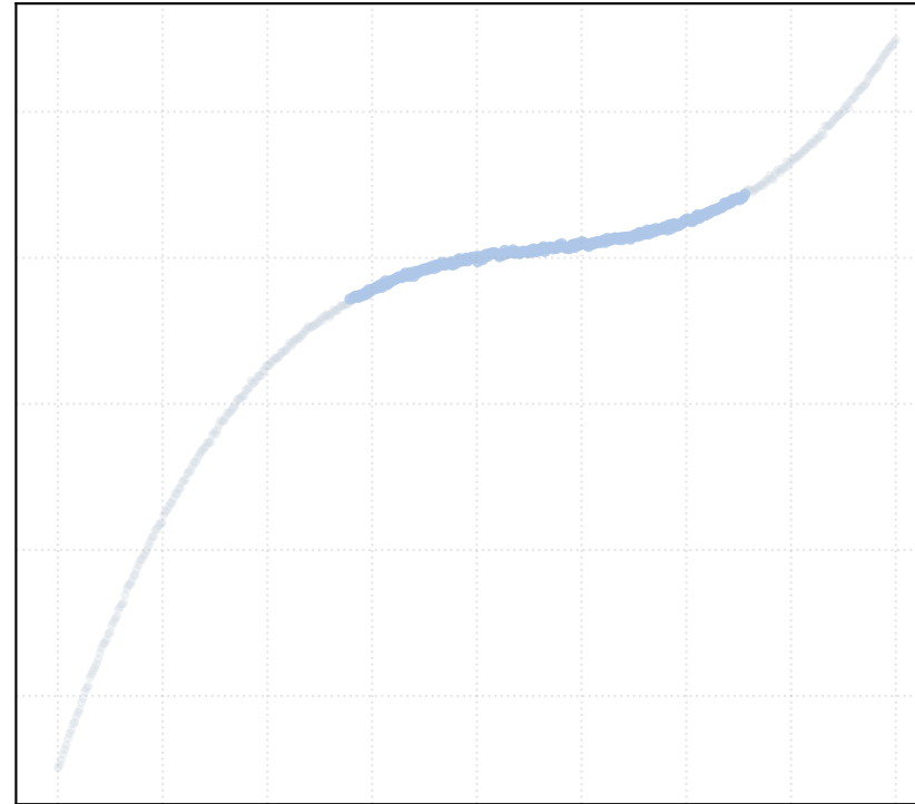
t_percentile = 0.4 [1 Clusters]
