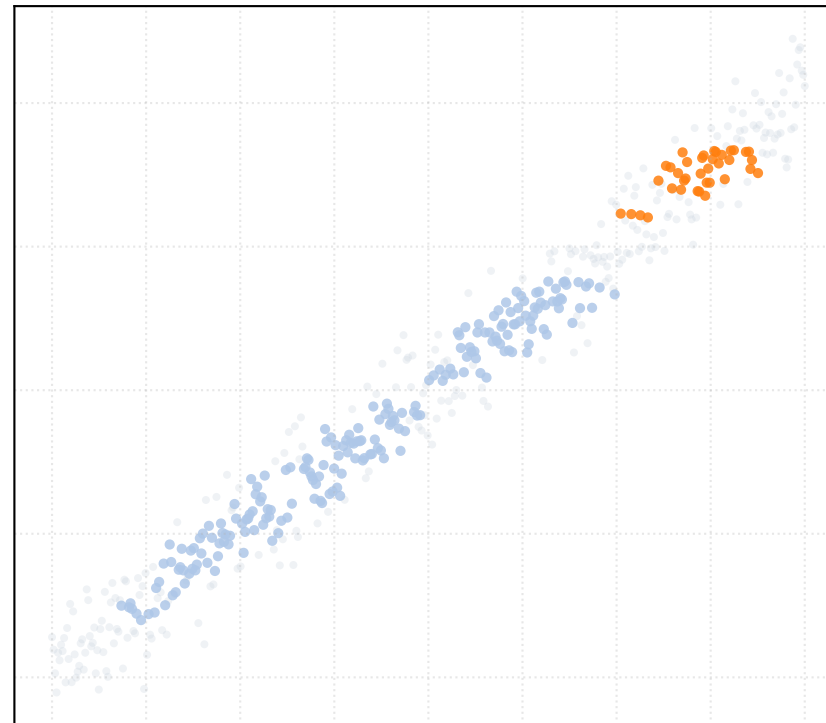
t_percentile = 0.4 [1 Clusters]
