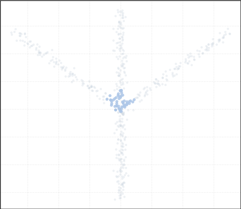
t_percentile = 0.3 [12 Clusters]
