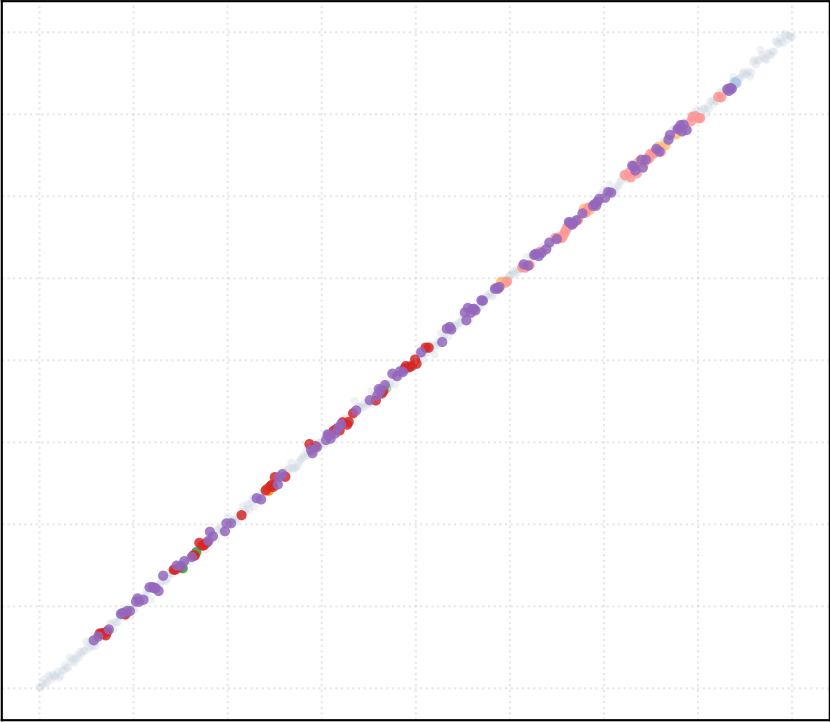
t_percentile = 0.25 [8 Clusters]
