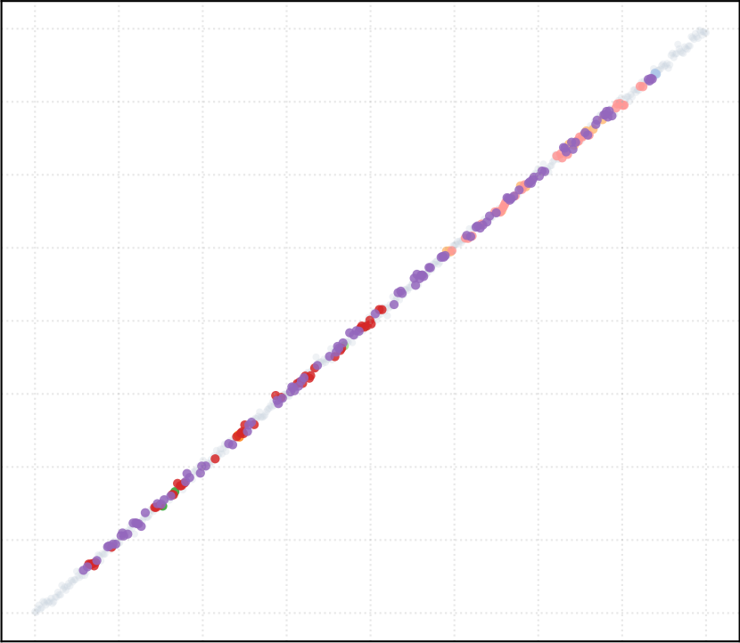
t_percentile = 0.3 [8 Clusters]
