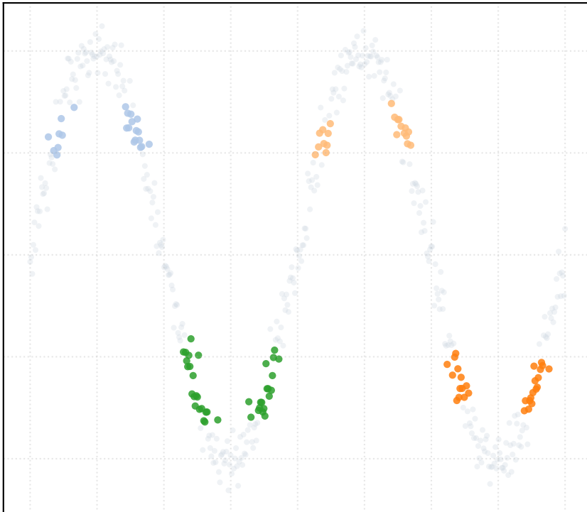
t_percentile = 0.25 [4 Clusters]
