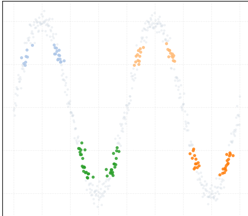
t_percentile = 0.3 [4 Clusters]
