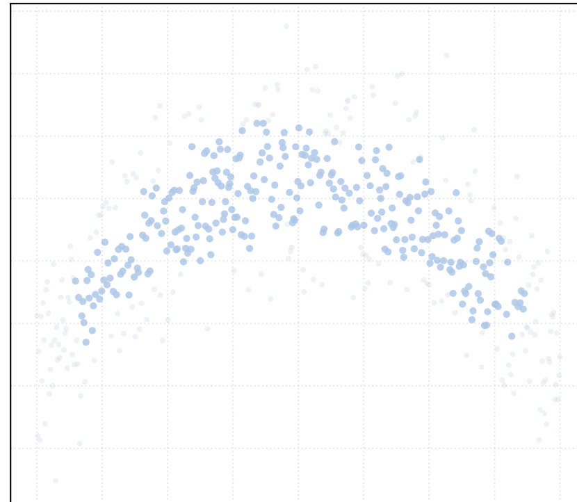
t_percentile = 0.5 [1 Clusters]
