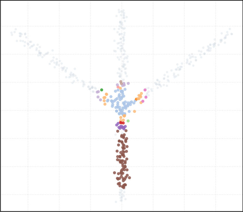
t_percentile = 0.3 [12 Clusters]
