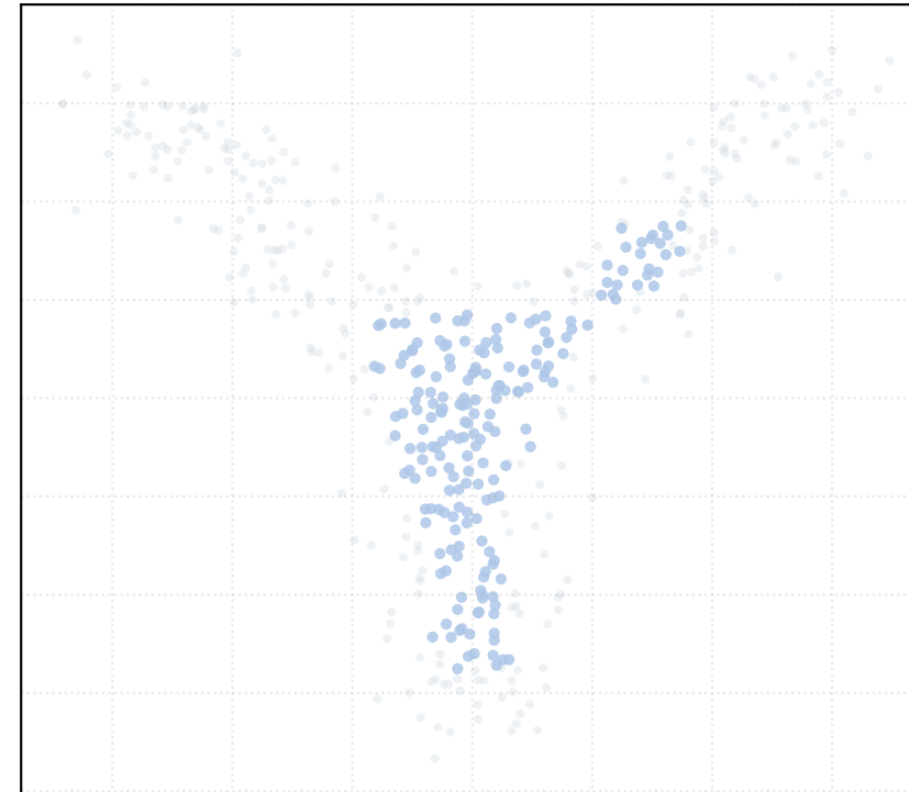
t_percentile = 0.5 [2 Clusters]
