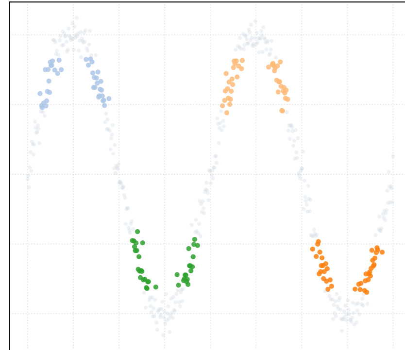
t_percentile = 0.5 [4 Clusters]
