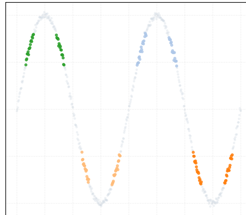
t_percentile = 0.5 [4 Clusters]
