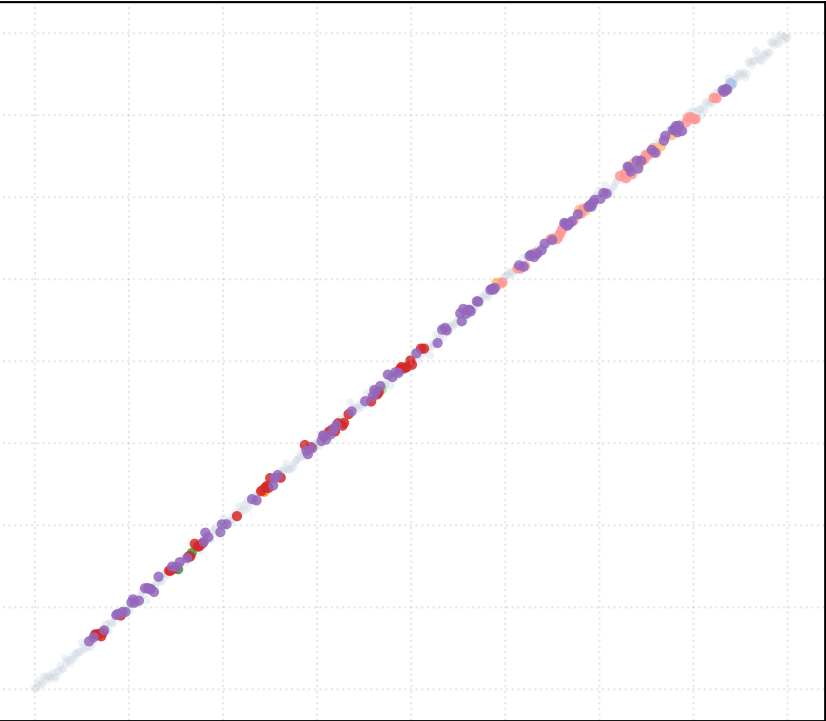
t_percentile = 0.5 [9 Clusters]
