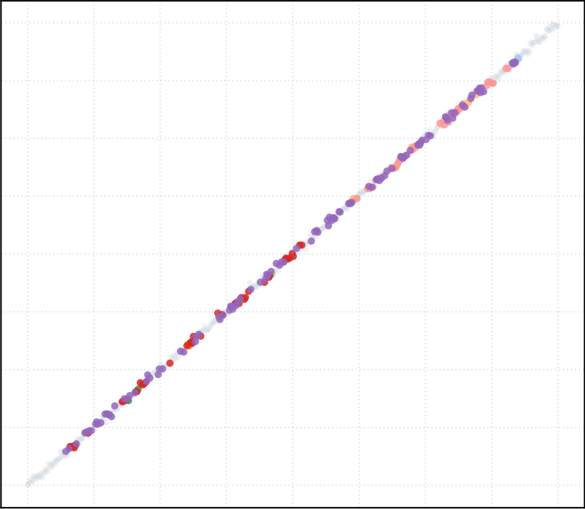
t_percentile = 0.4 [8 Clusters]
