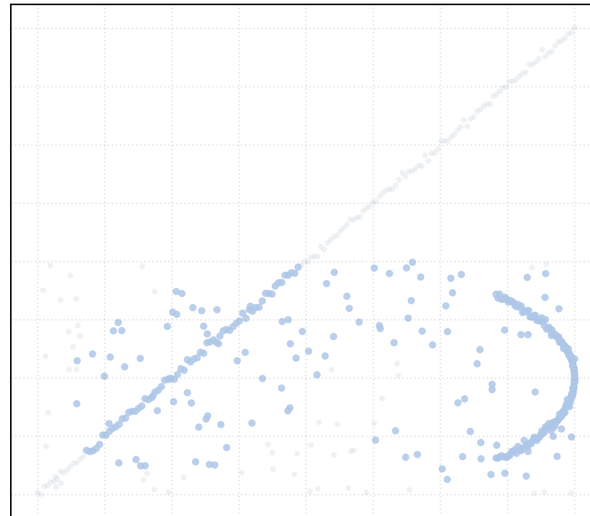
t_percentile = 0.5 [1 Clusters]
