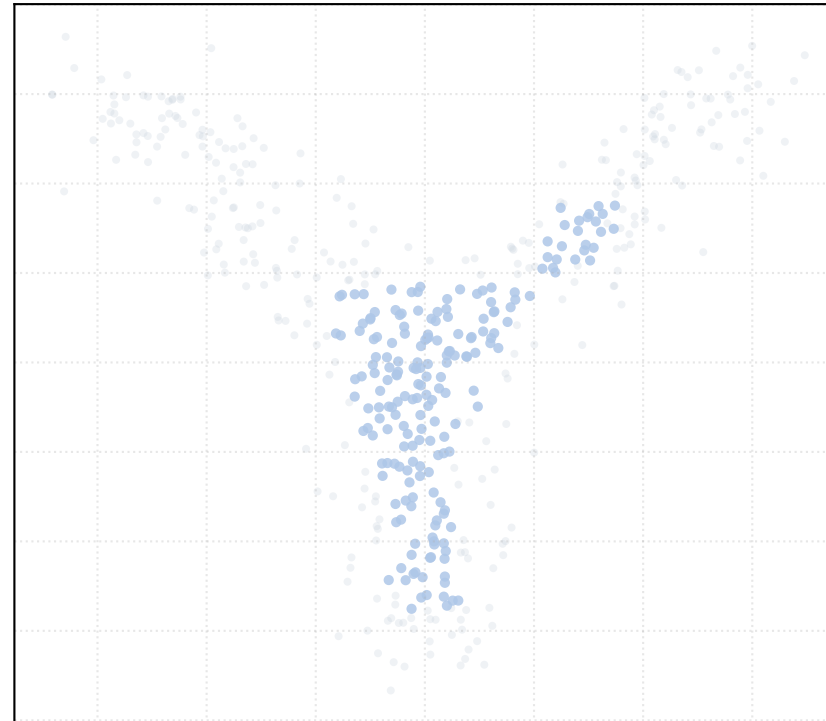
t_percentile = 0.4 [2 Clusters]
