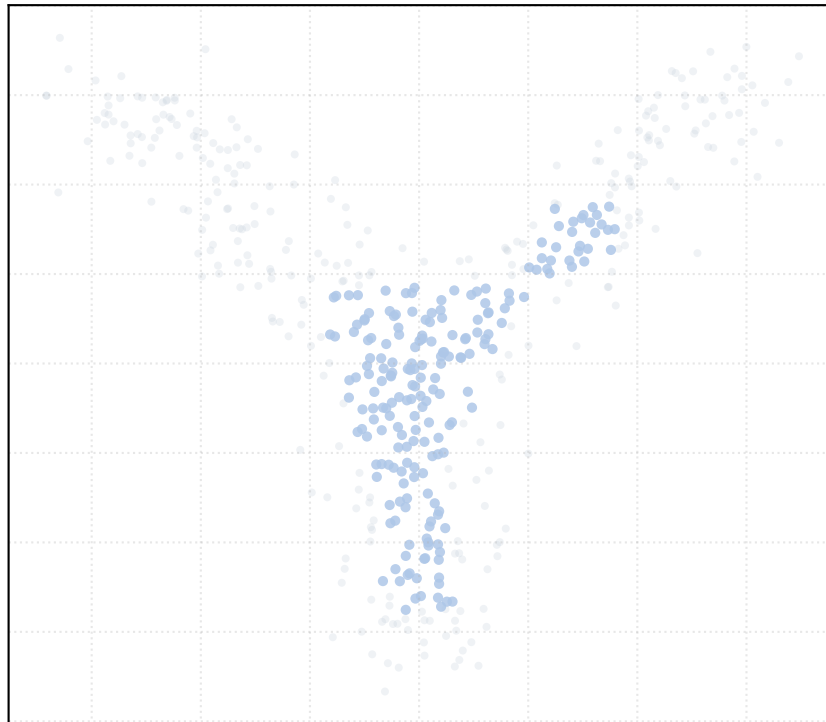
t_percentile = 0.3 [1 Clusters]
