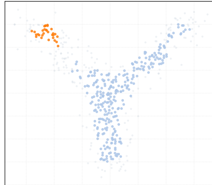
t_percentile = 0.5 [2 Clusters]
