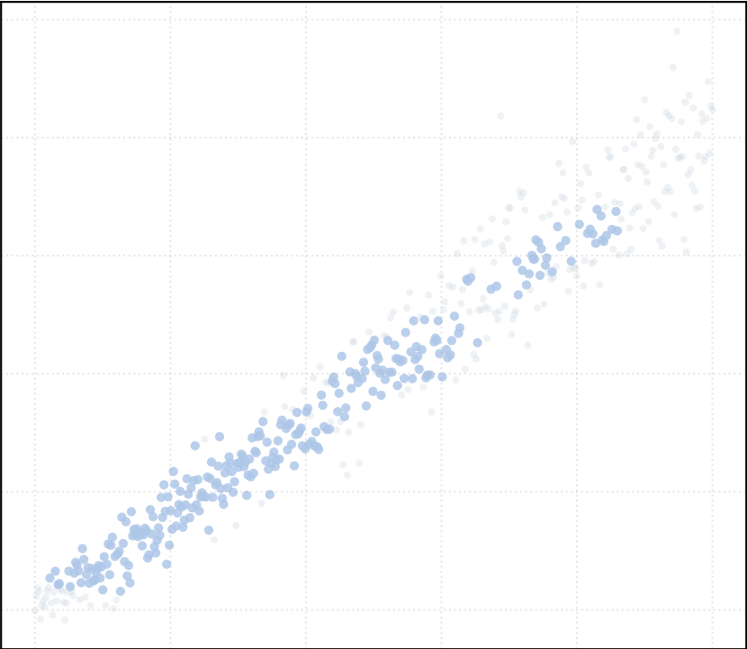
t_percentile = 0.5 [1 Clusters]
