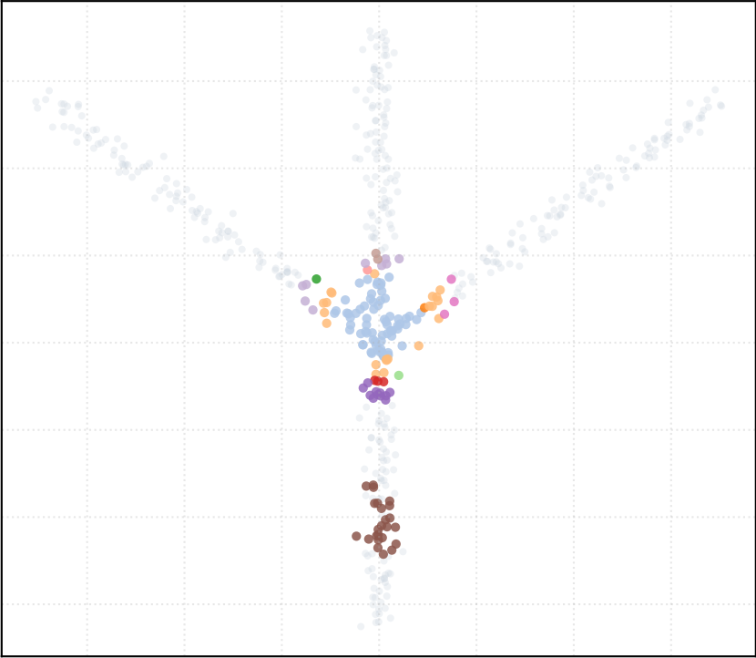
t_percentile = 0.25 [12 Clusters]
