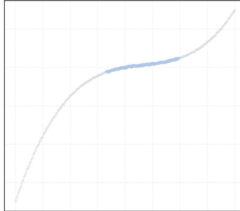
t_percentile = 0.5 [1 Clusters]
