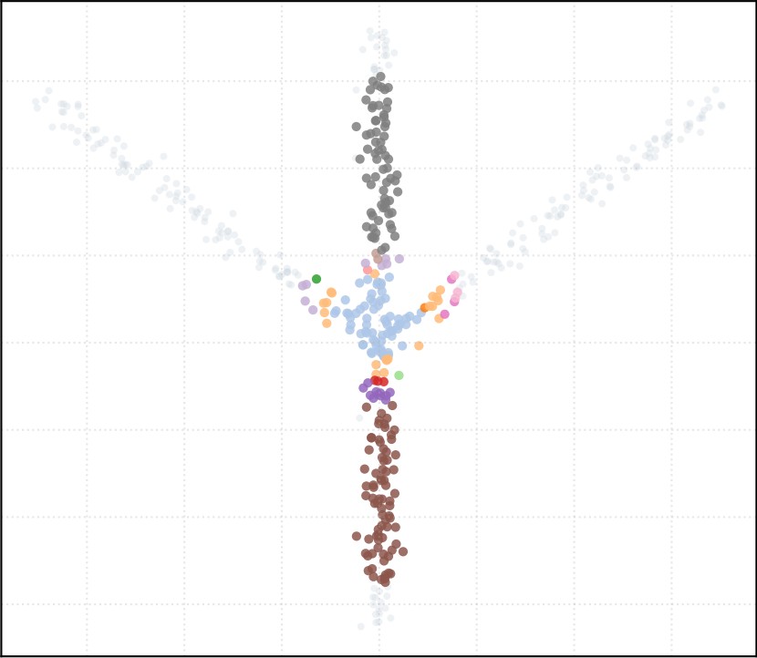
t_percentile = 0.4 [14 Clusters]
