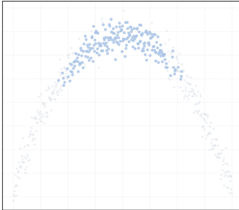
t_percentile = 0.3 [1 Clusters]
