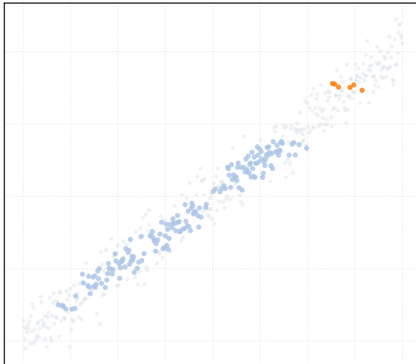
t_percentile = 0.3 [2 Clusters]
