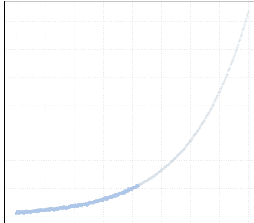
t_percentile = 0.4 [1 Clusters]
