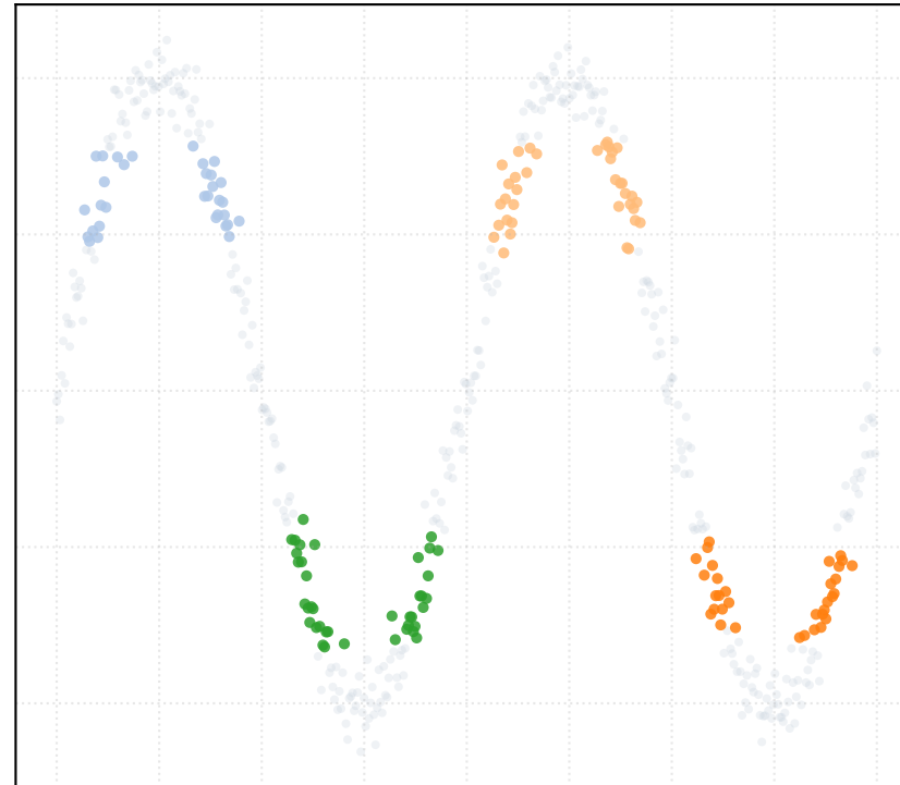
t_percentile = 0.4 [4 Clusters]
