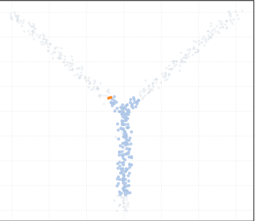
t_percentile = 0.5 [7 Clusters]
