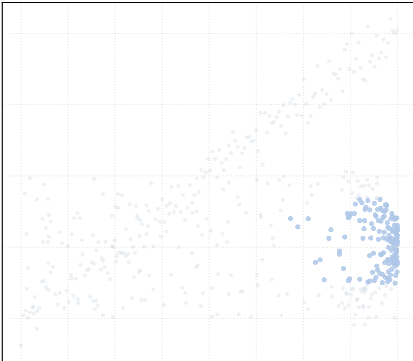
t_percentile = 0.25 [1 Clusters]
