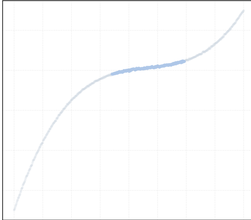
t_percentile = 0.3 [1 Clusters]
