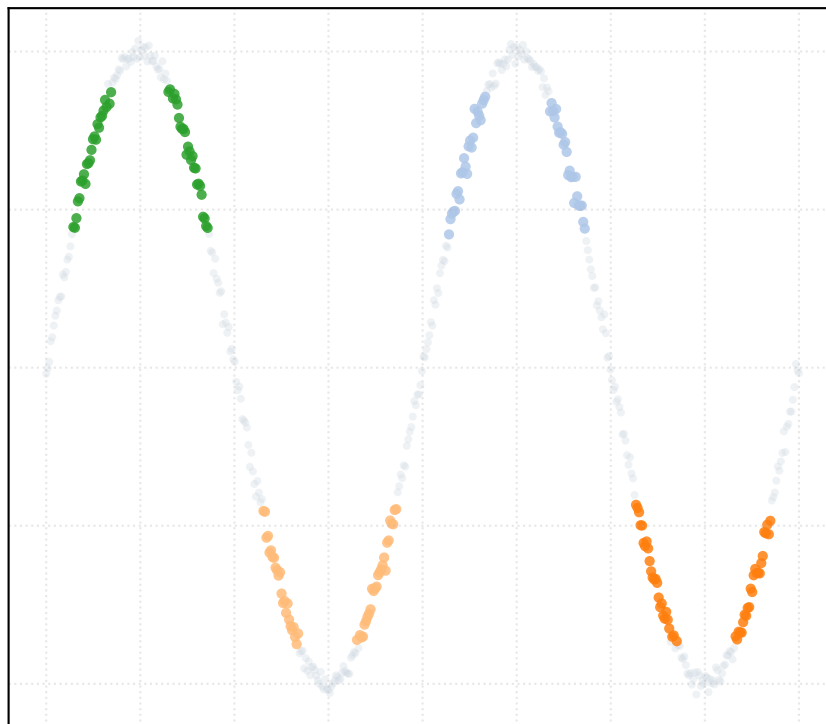
t_percentile = 0.3 [4 Clusters]
