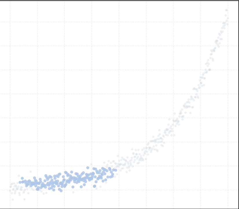
t_percentile = 0.5 [1 Clusters]
