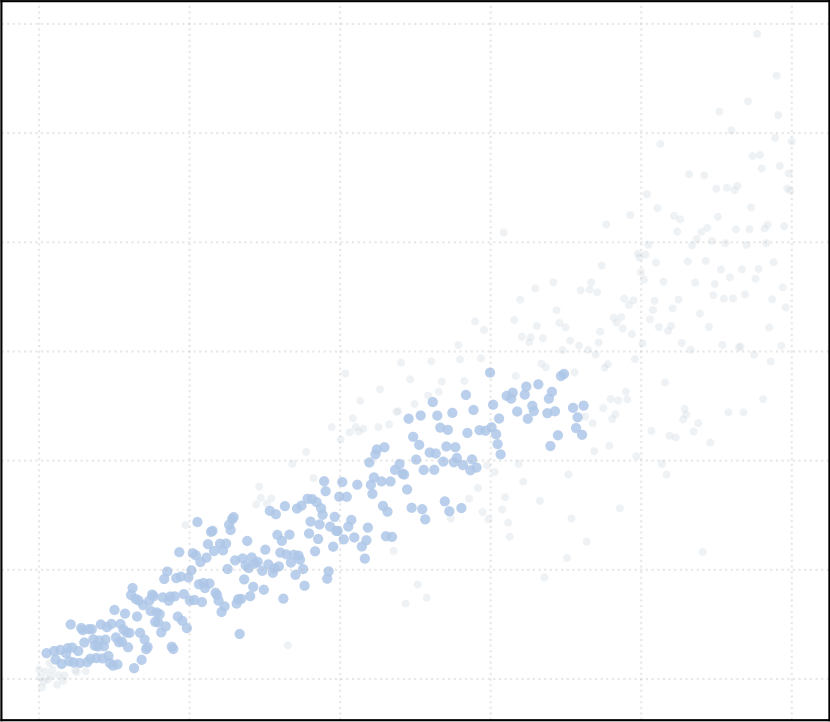
t_percentile = 0.4 [1 Clusters]
