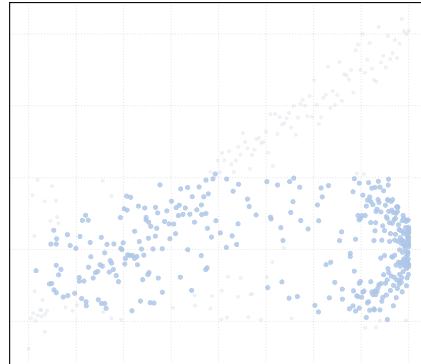
t_percentile = 0.5 [1 Clusters]
