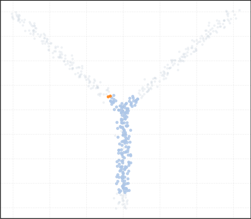
t_percentile = 0.25 [2 Clusters]
