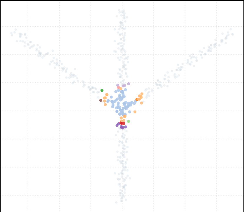
t_percentile = 0.5 [15 Clusters]
