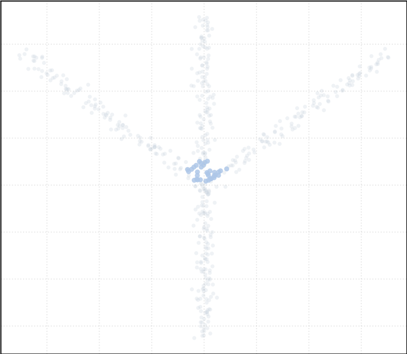
t_percentile = 0.25 [12 Clusters]
