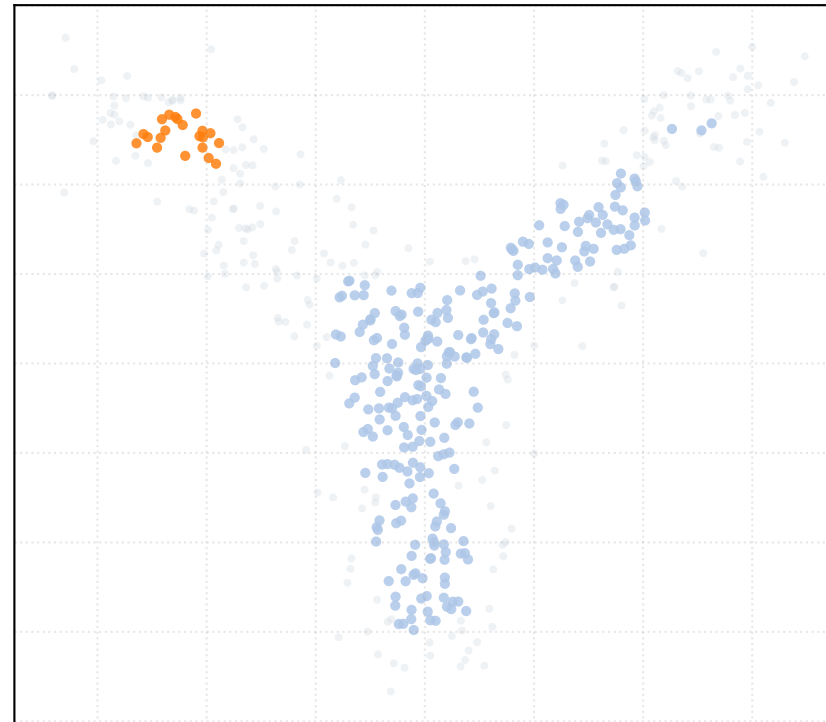
t_percentile = 0.4 [2 Clusters]
