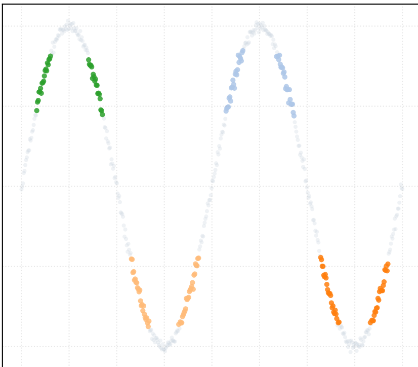
t_percentile = 0.25 [4 Clusters]
