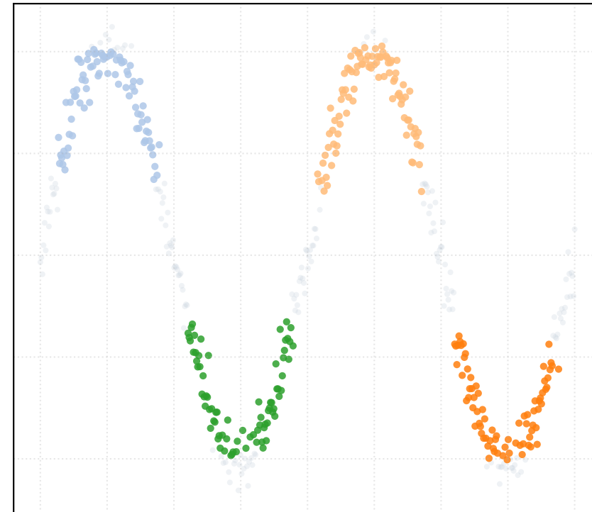
t_percentile = 0.5 [4 Clusters]
