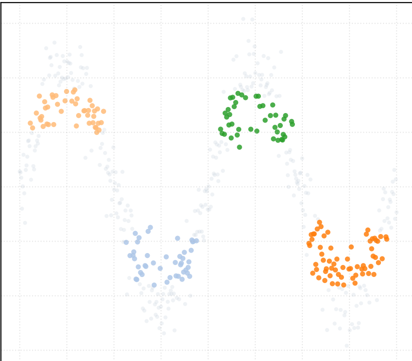
t_percentile = 0.25 [4 Clusters]
