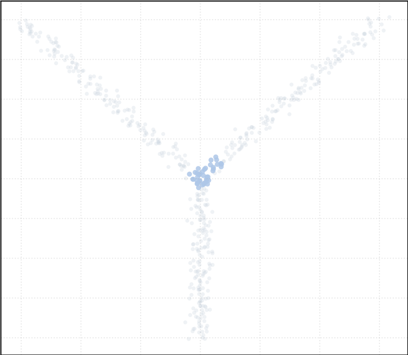
t_percentile = 0.25 [2 Clusters]
