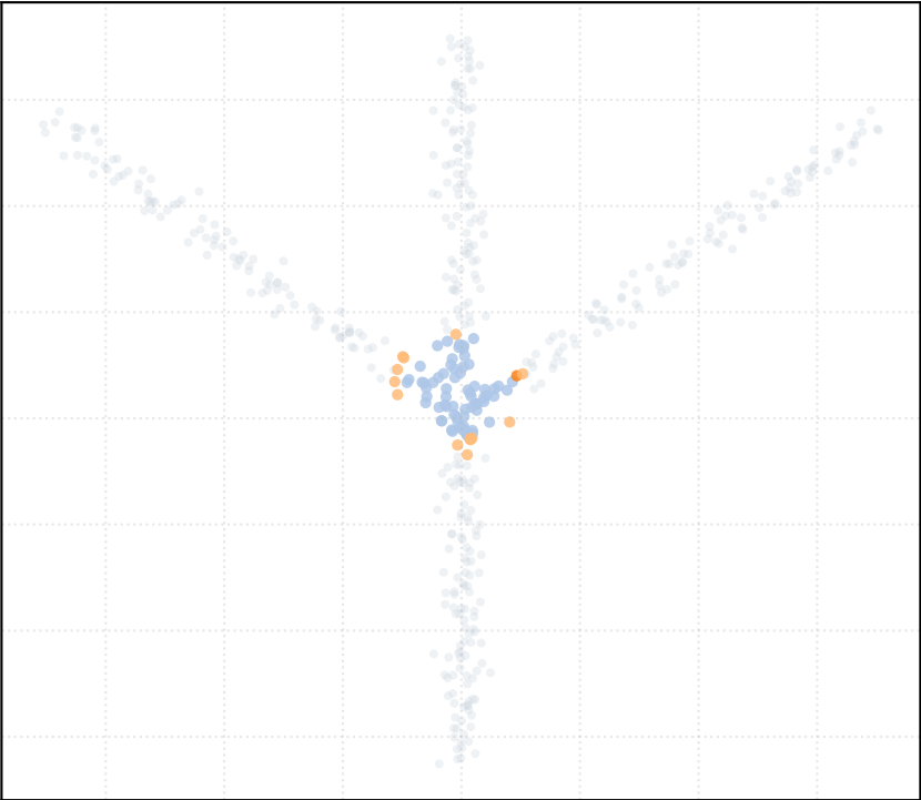
t_percentile = 0.4 [14 Clusters]
