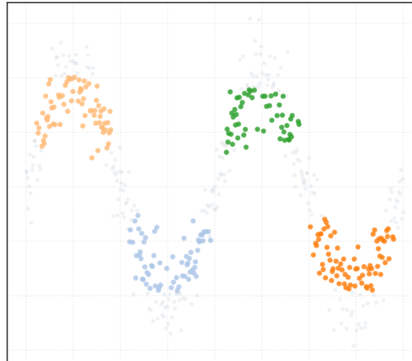
t_percentile = 0.4 [4 Clusters]
