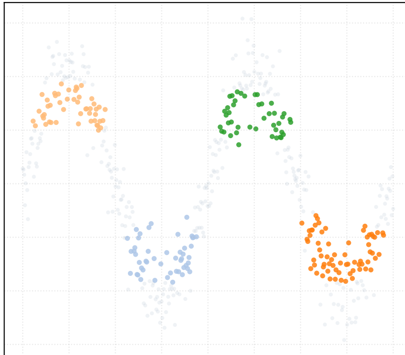
t_percentile = 0.3 [4 Clusters]
