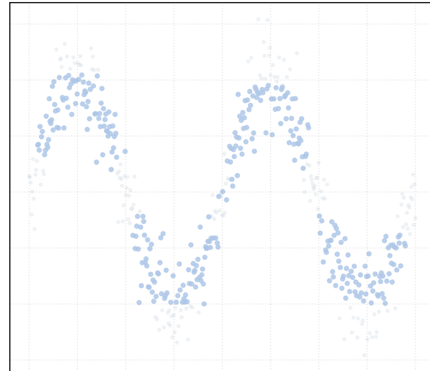
t_percentile = 0.5 [1 Clusters]
