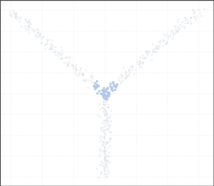
t_percentile = 0.3 [2 Clusters]
