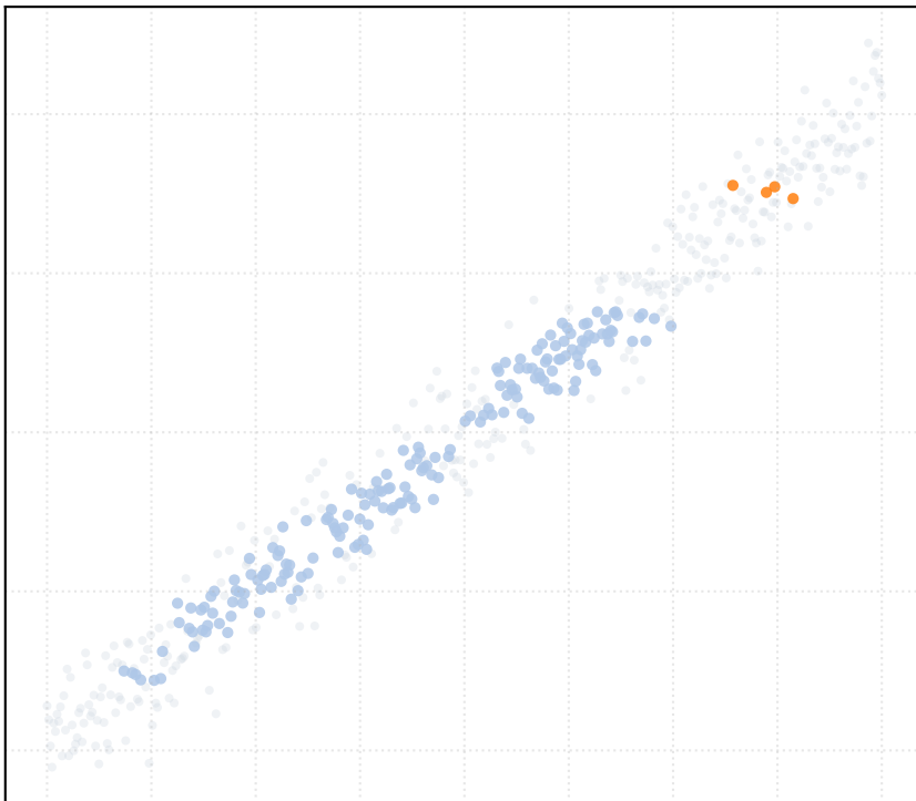
t_percentile = 0.25 [2 Clusters]
