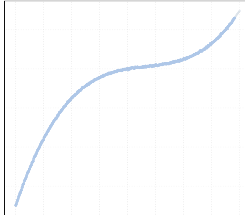
t_percentile = 0.5 [1 Clusters]
