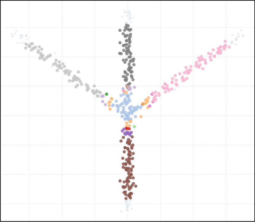
t_percentile = 0.5 [15 Clusters]
