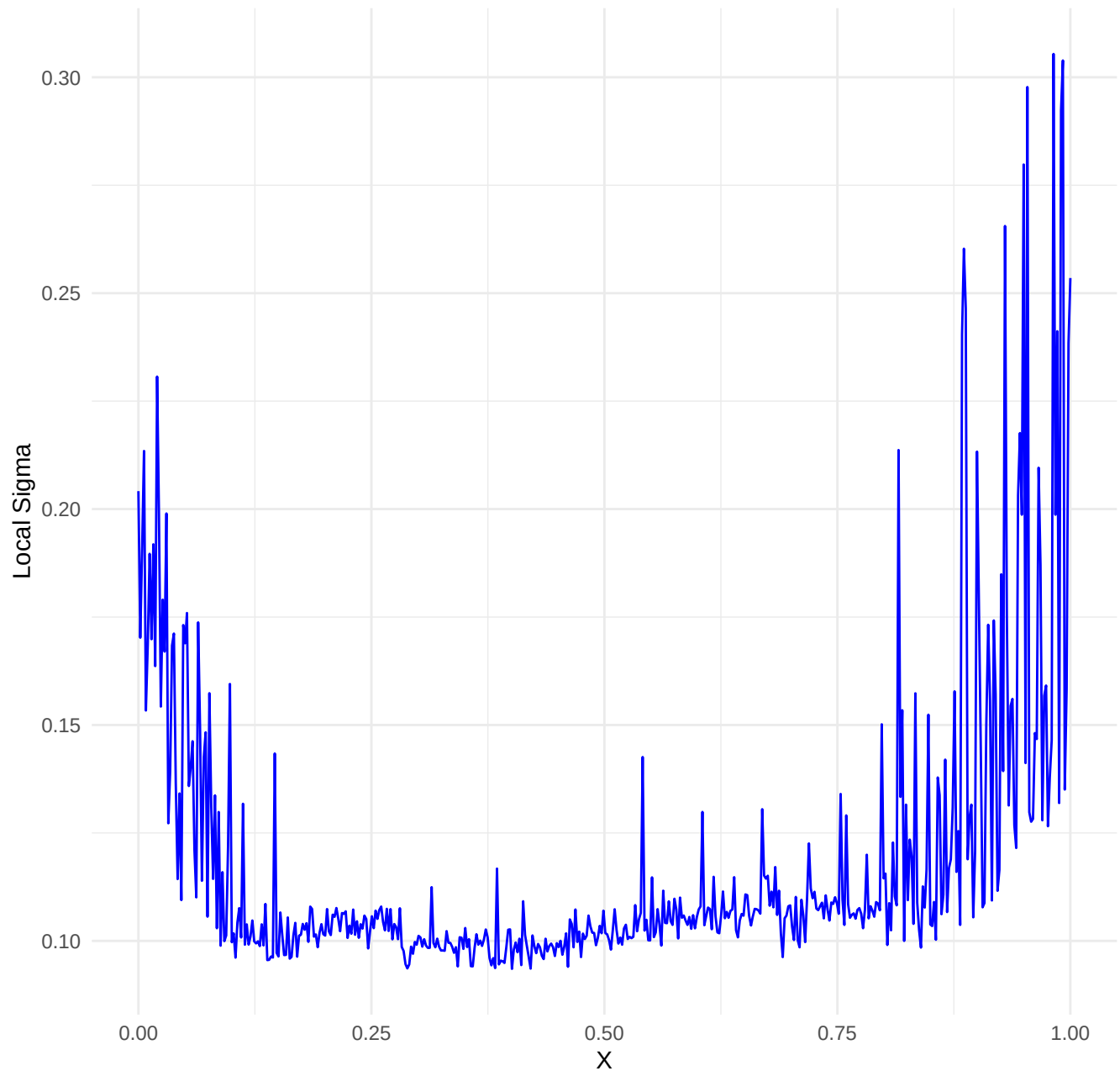
Dataset: heteroscedastic_noise_medium | k= 200 , iter= 21
