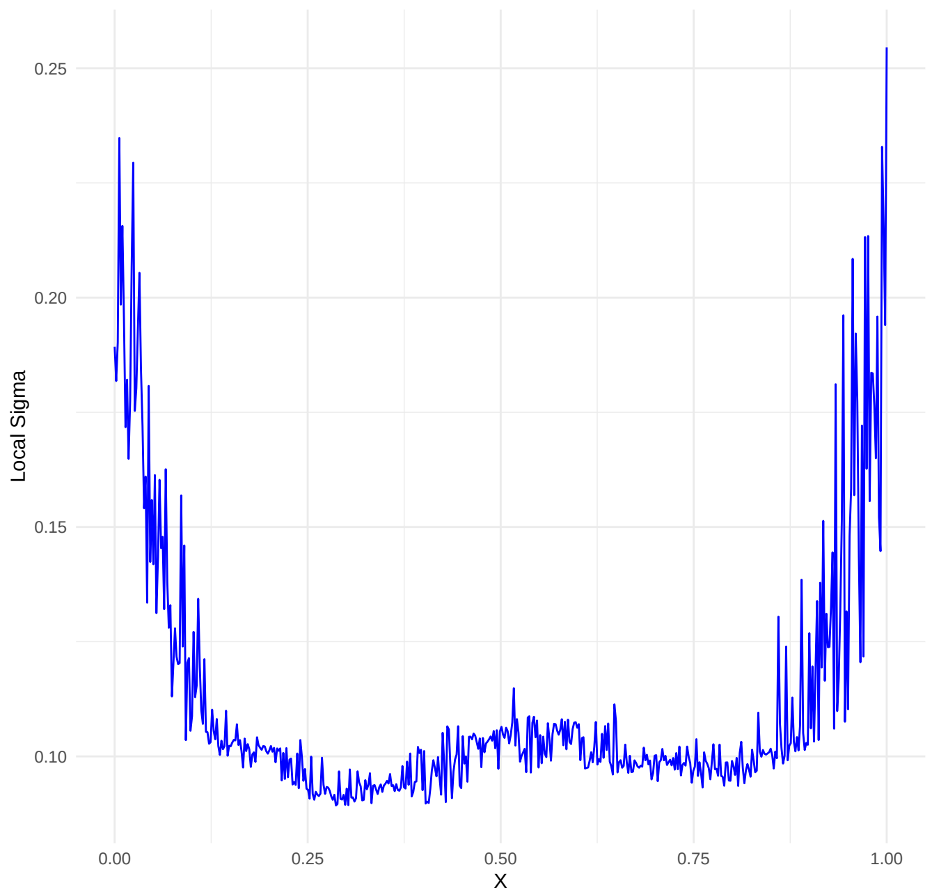
Dataset: heteroscedastic_noise_low | k= 200 , iter= 21
