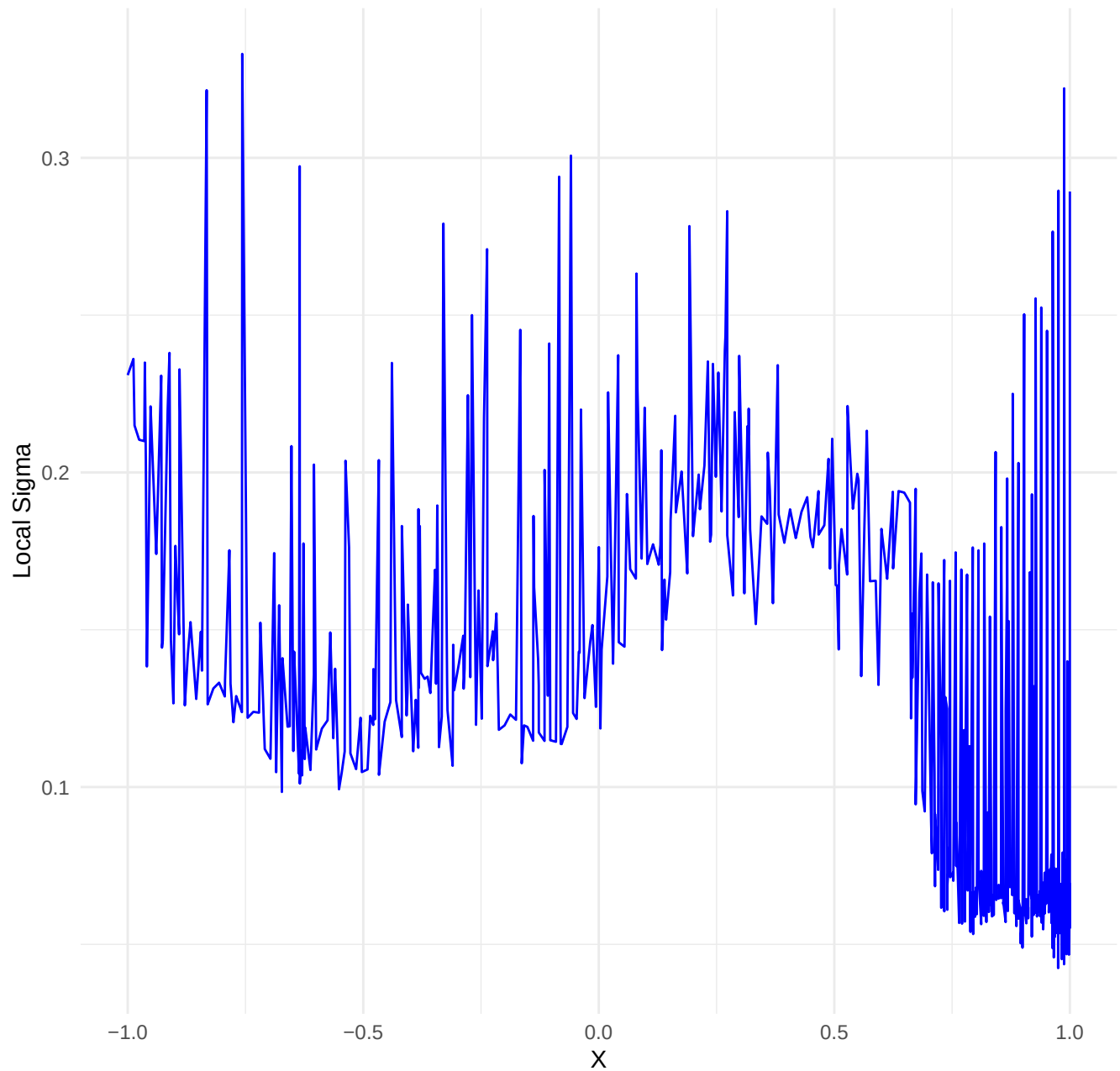
Dataset: mixed_generators_noise_medium | k= 50 , iter= 21
