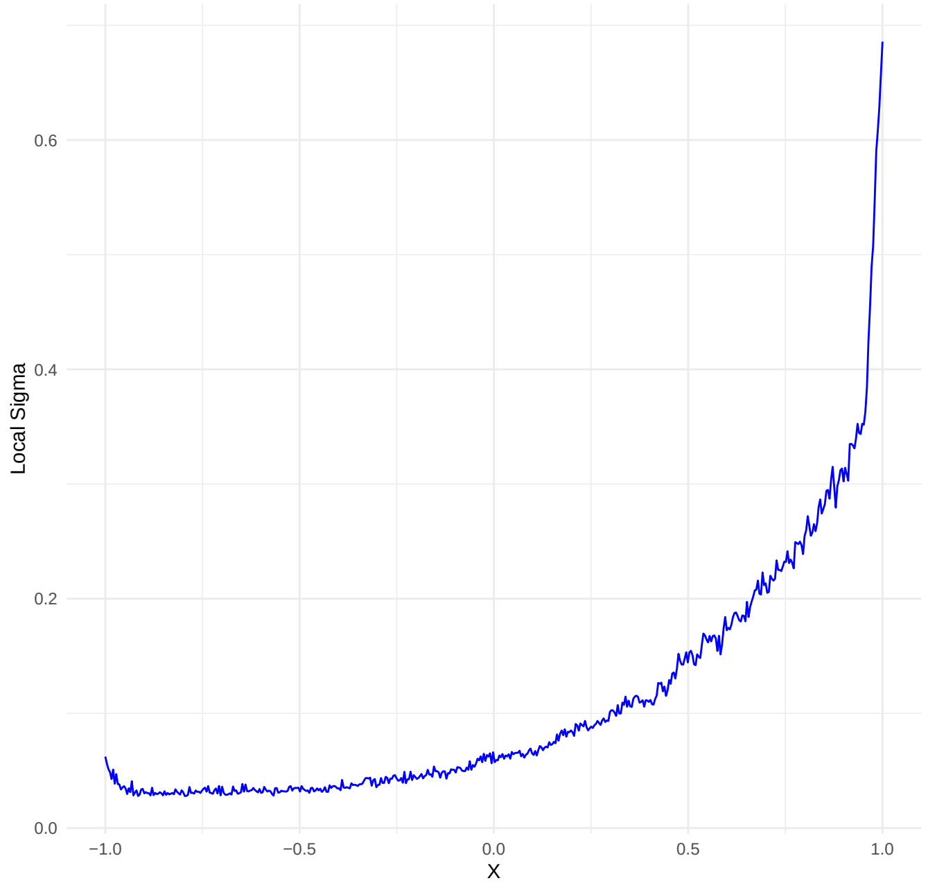
Dataset: exponential_noise_low | k= 50 , iter= 21
