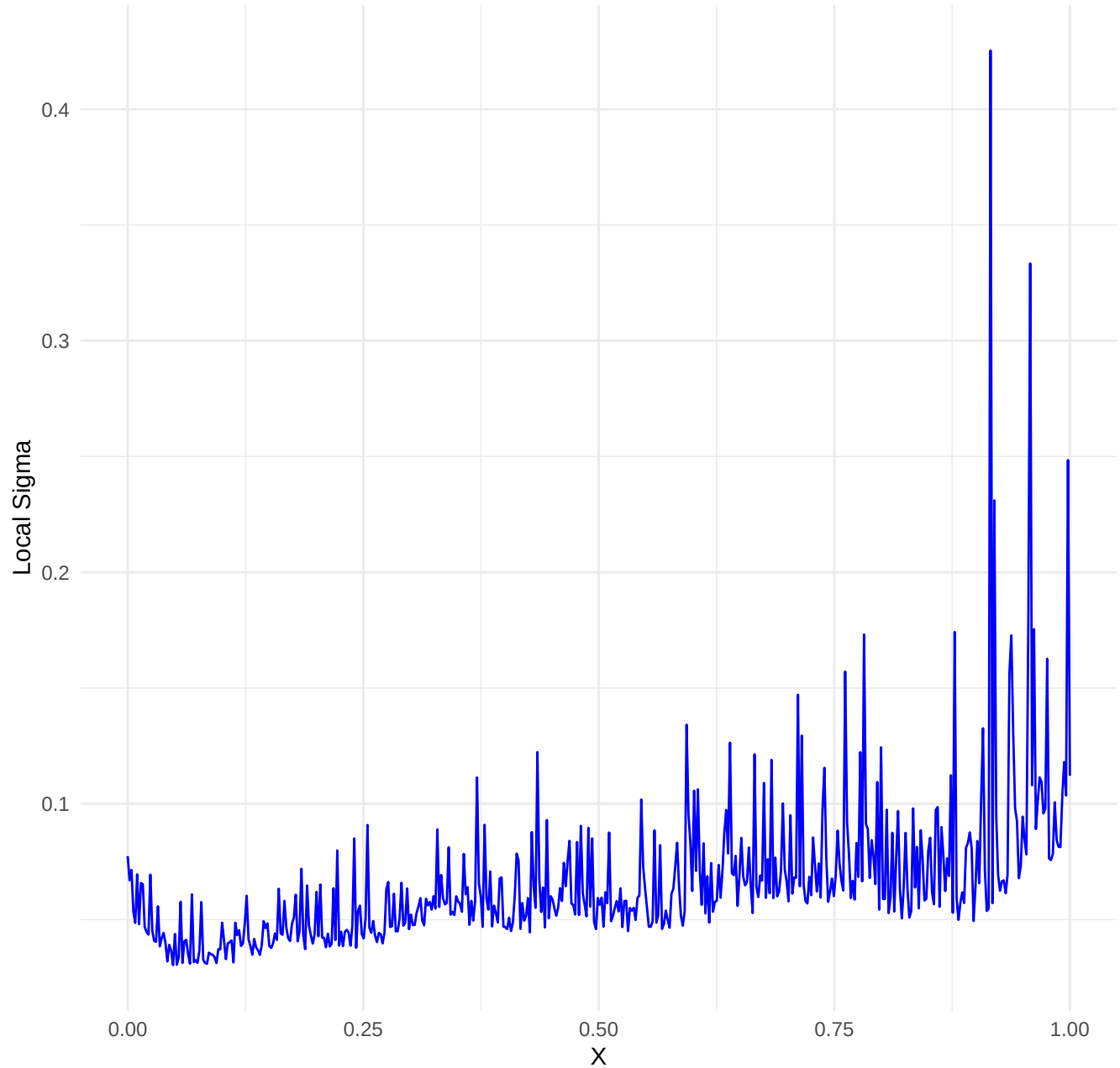
Dataset: heteroscedastic_noise_high | k= 50 , iter= 21
