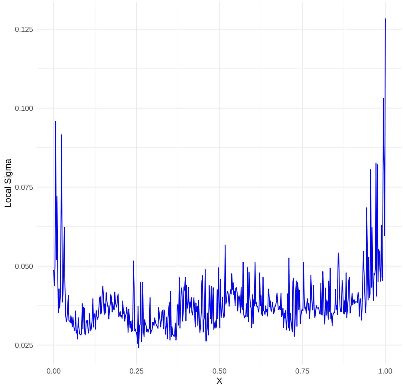
Dataset: heteroscedastic_noise_low | k= 50 , iter= 21
