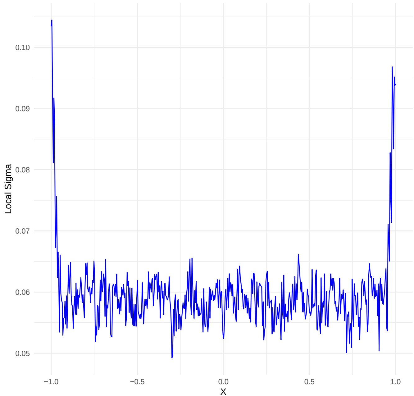
Dataset: linear_noise_low | k= 50 , iter= 21
