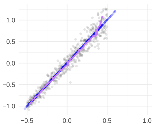
ManLe
