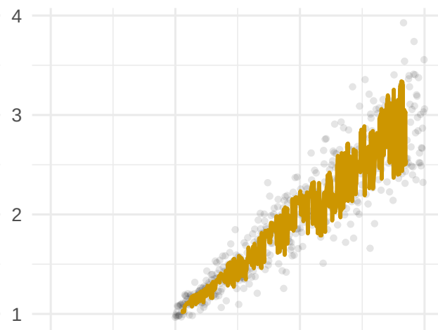
ANWIL (mode 2)
