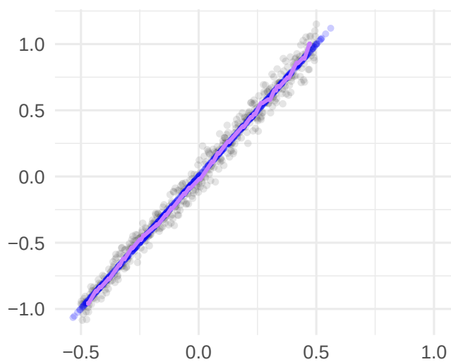
ManLe
