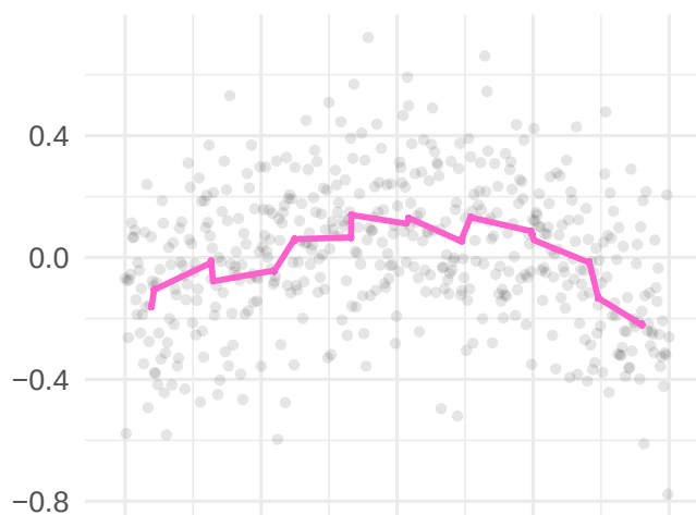
ANWIL (mode 1)
