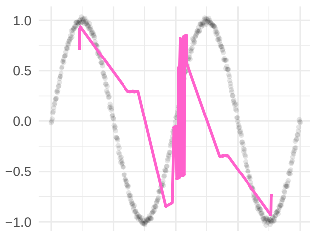
ANWIL (mode 1)
