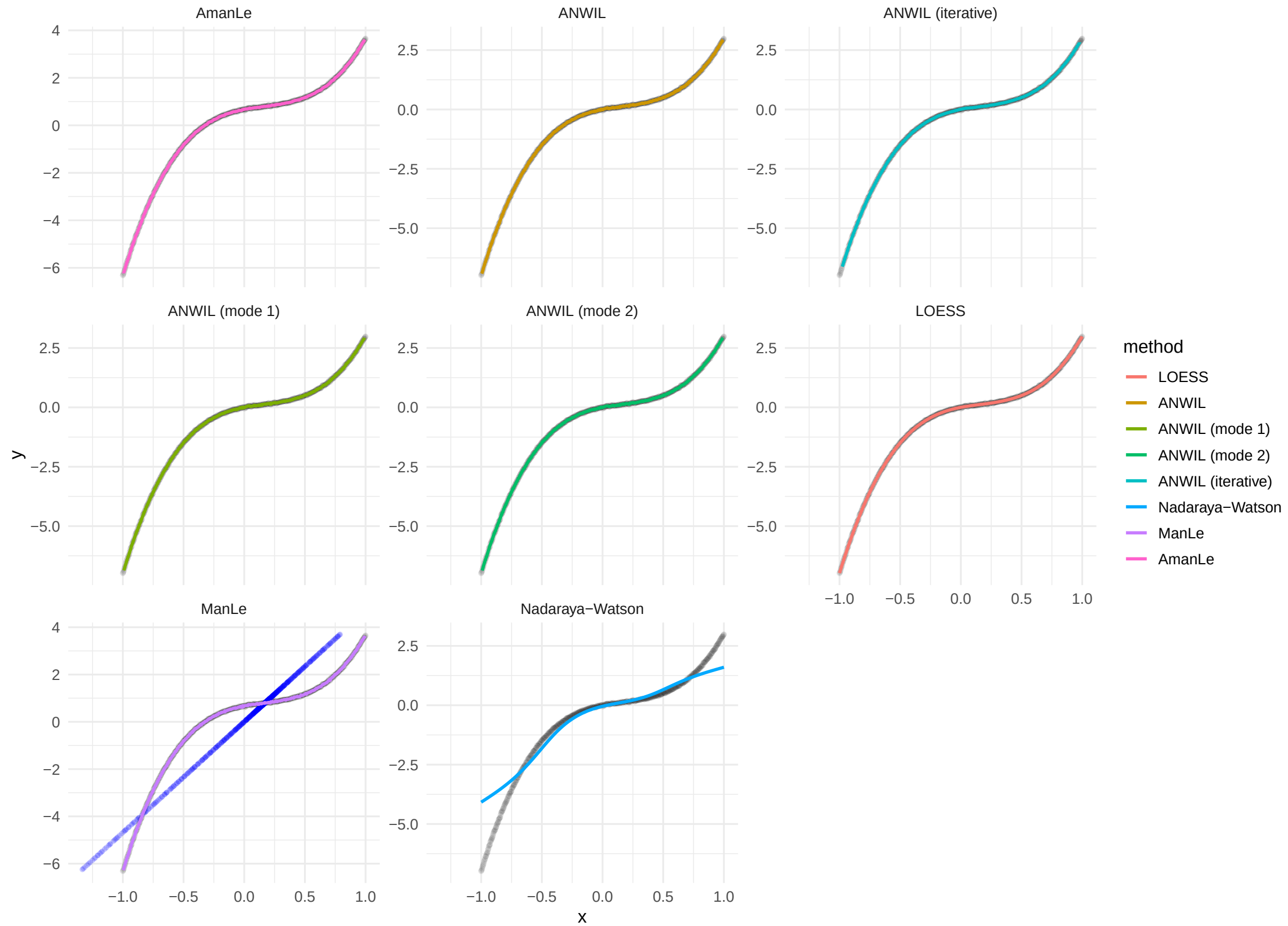
cubic_noise_low_smoothed_k5_iter20
