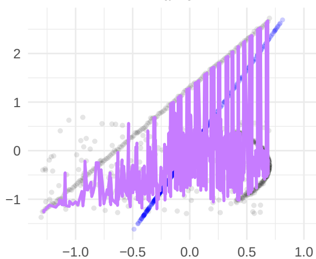
ManLe
