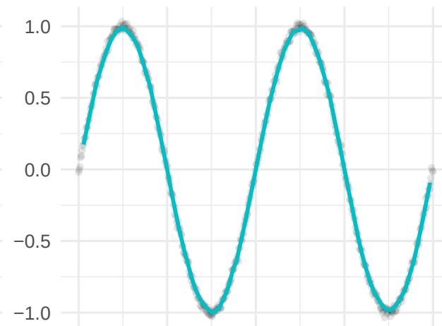
ANWIL (iterative)
