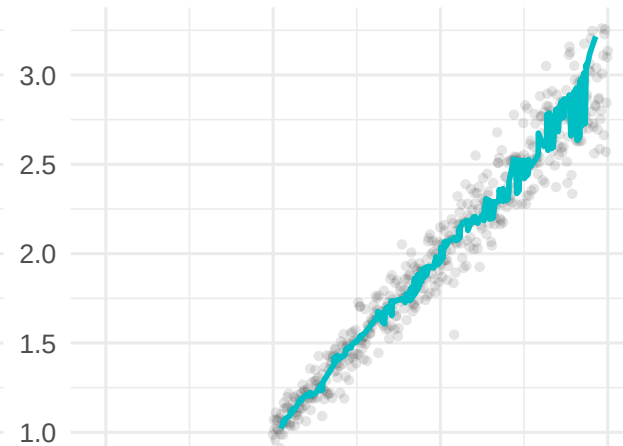
ANWIL (iterative)
