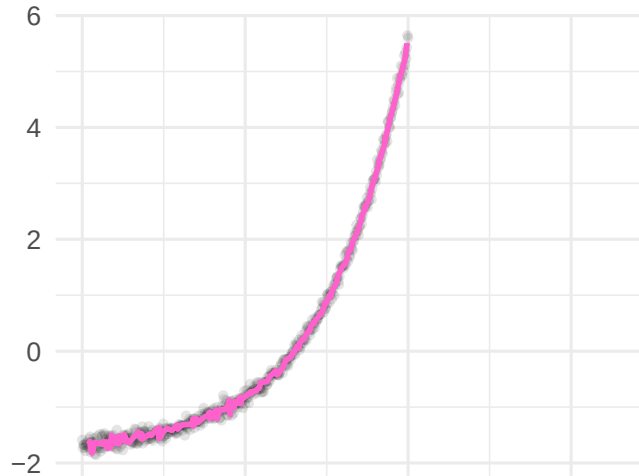
ANWIL (mode 1)
