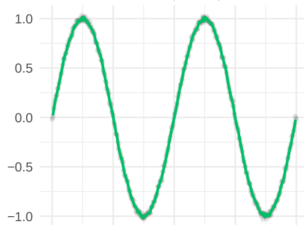
ANWIL (mode 2)
