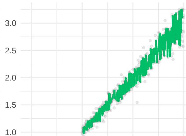
ANWIL (mode 2)
