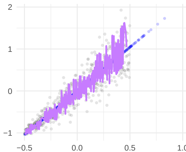
ManLe
