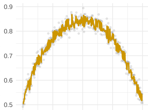
ANWIL (mode 2)
