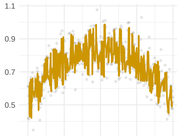
ANWIL (mode 2)
