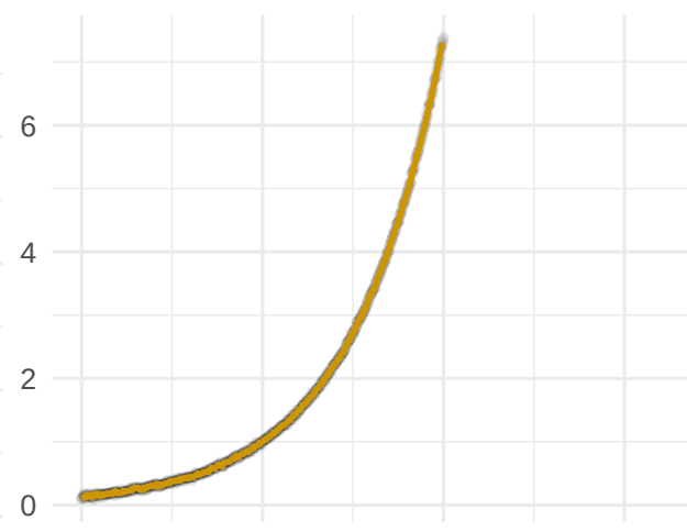
ANWIL (mode 2)
