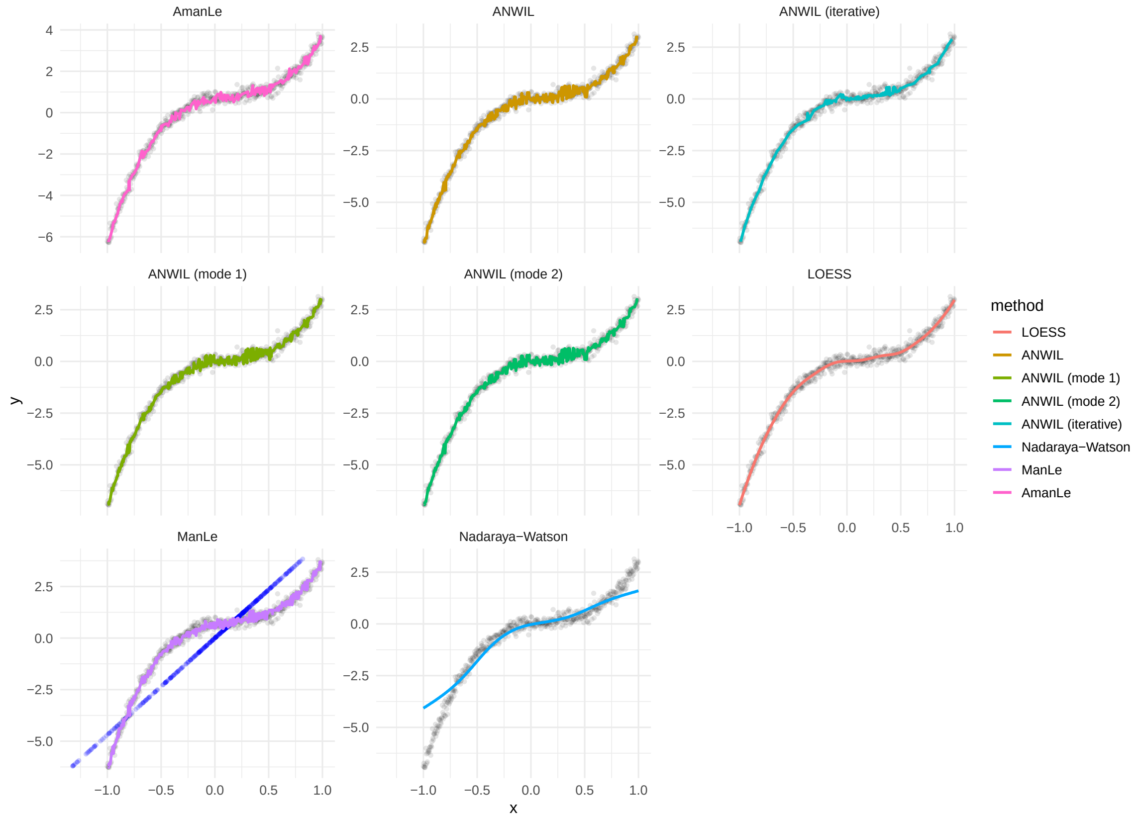
cubic_noise_high_smoothed_k5_iter20
