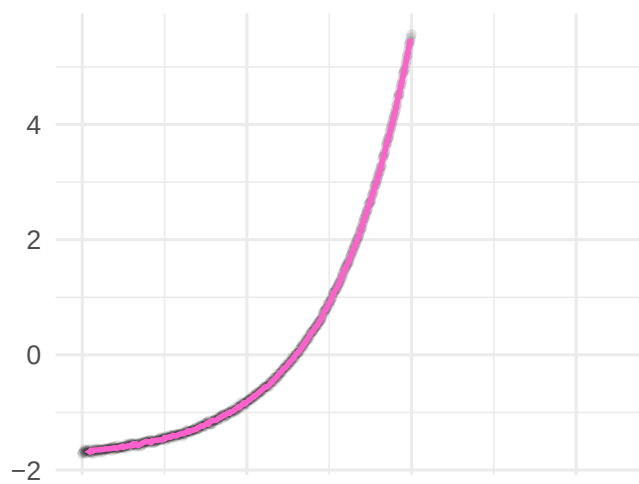
ANWIL (mode 1)
