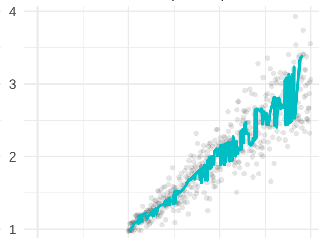
ANWIL (iterative)
