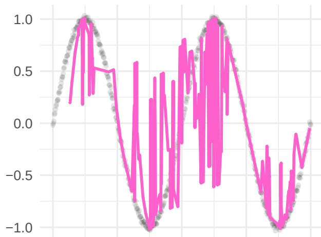
AmanLe
