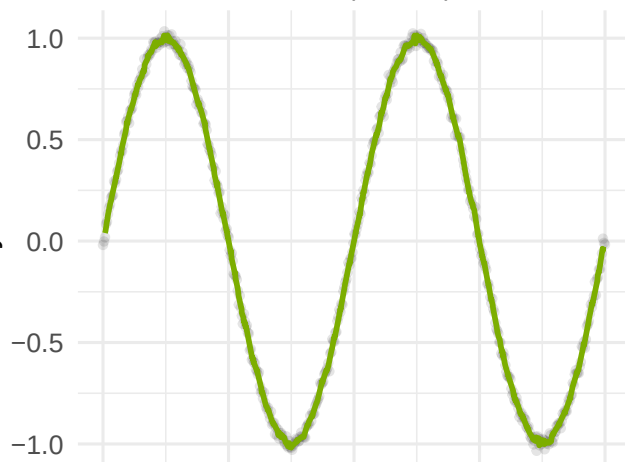
ANWIL (mode 1)
