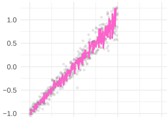
AmanLe
