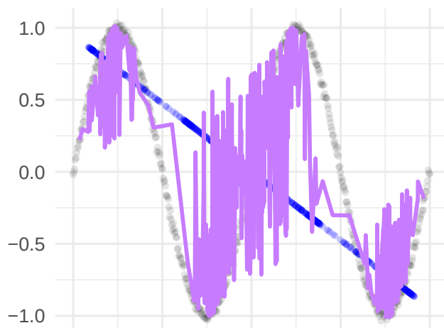
ManLe
