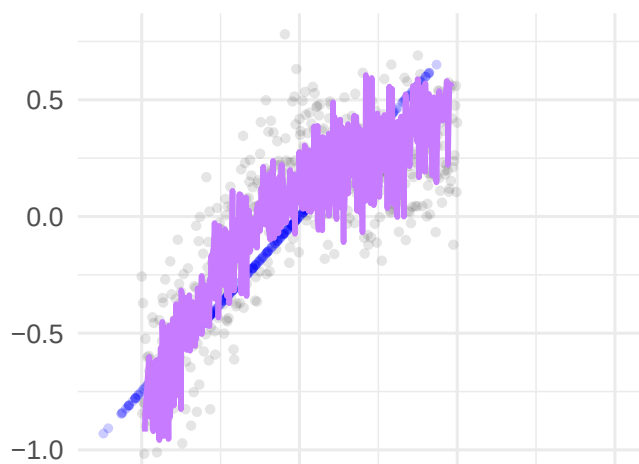
ManLe
