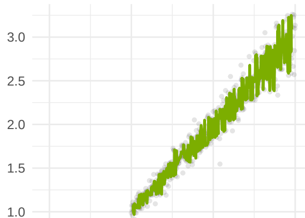
ANWIL (mode 1)
