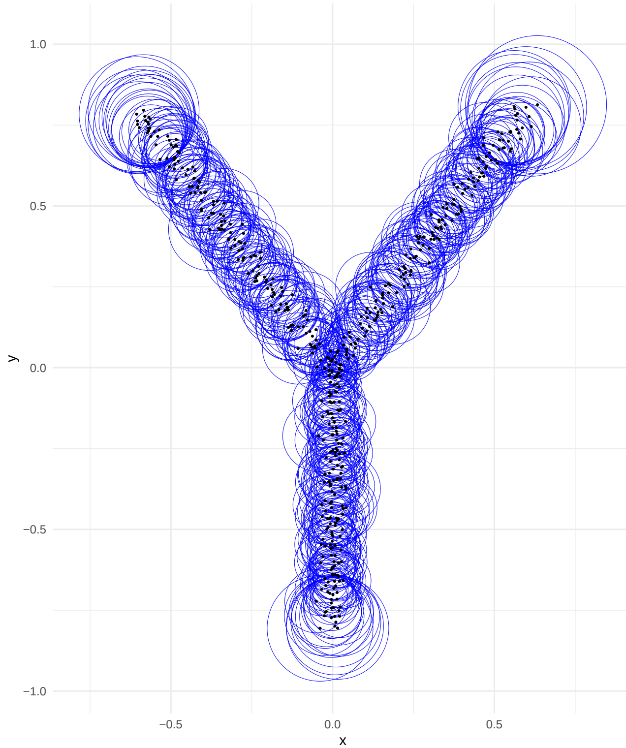
All Adaptive Spheres Visualizing local neighborhood size (radius) for every point.
