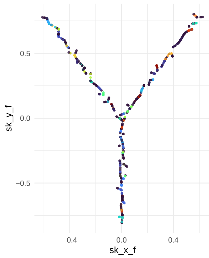
Converged
