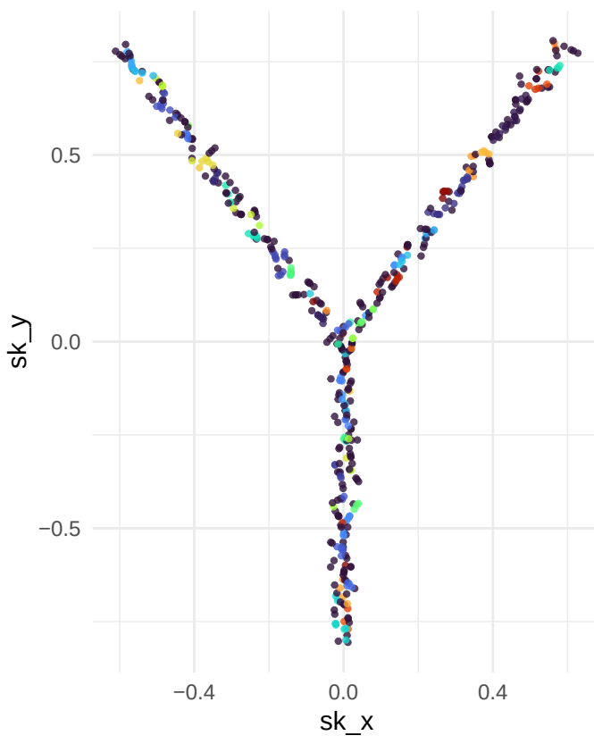
Iteration 1
