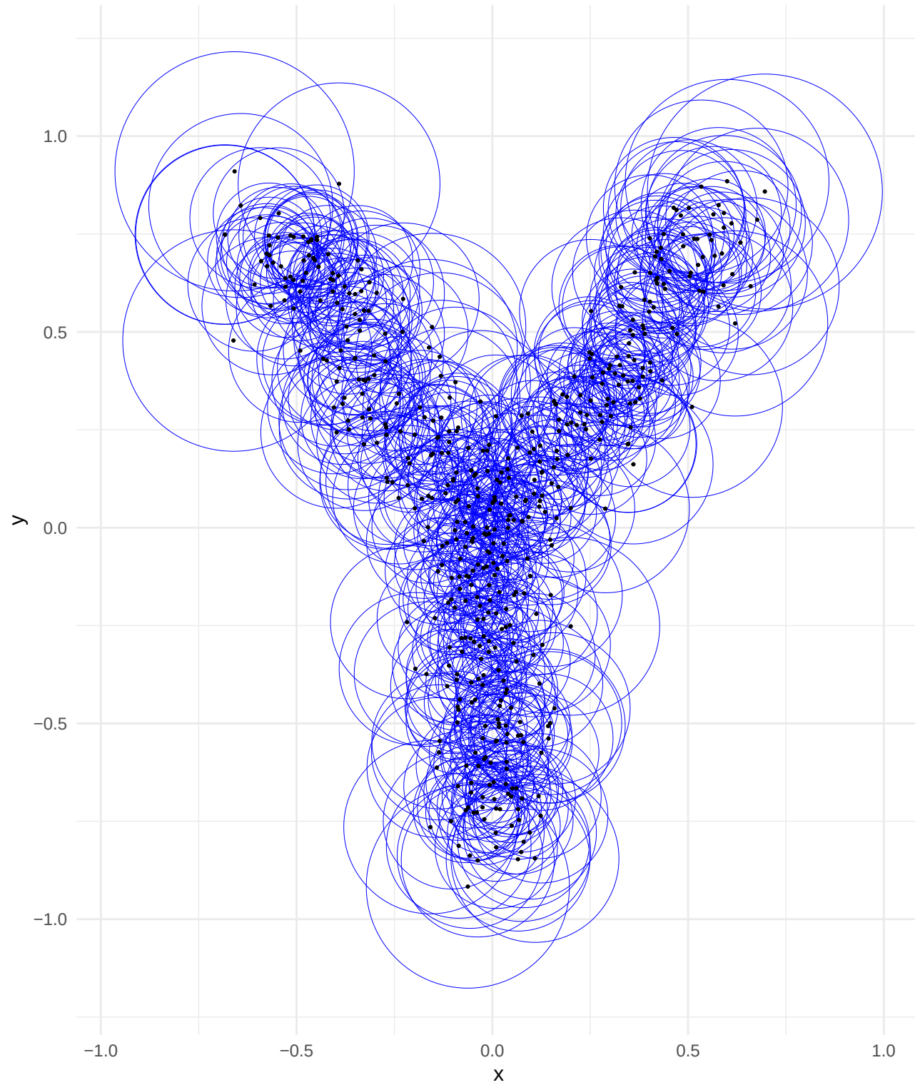
All Adaptive Spheres Visualizing local neighborhood size (radius) for every point.
