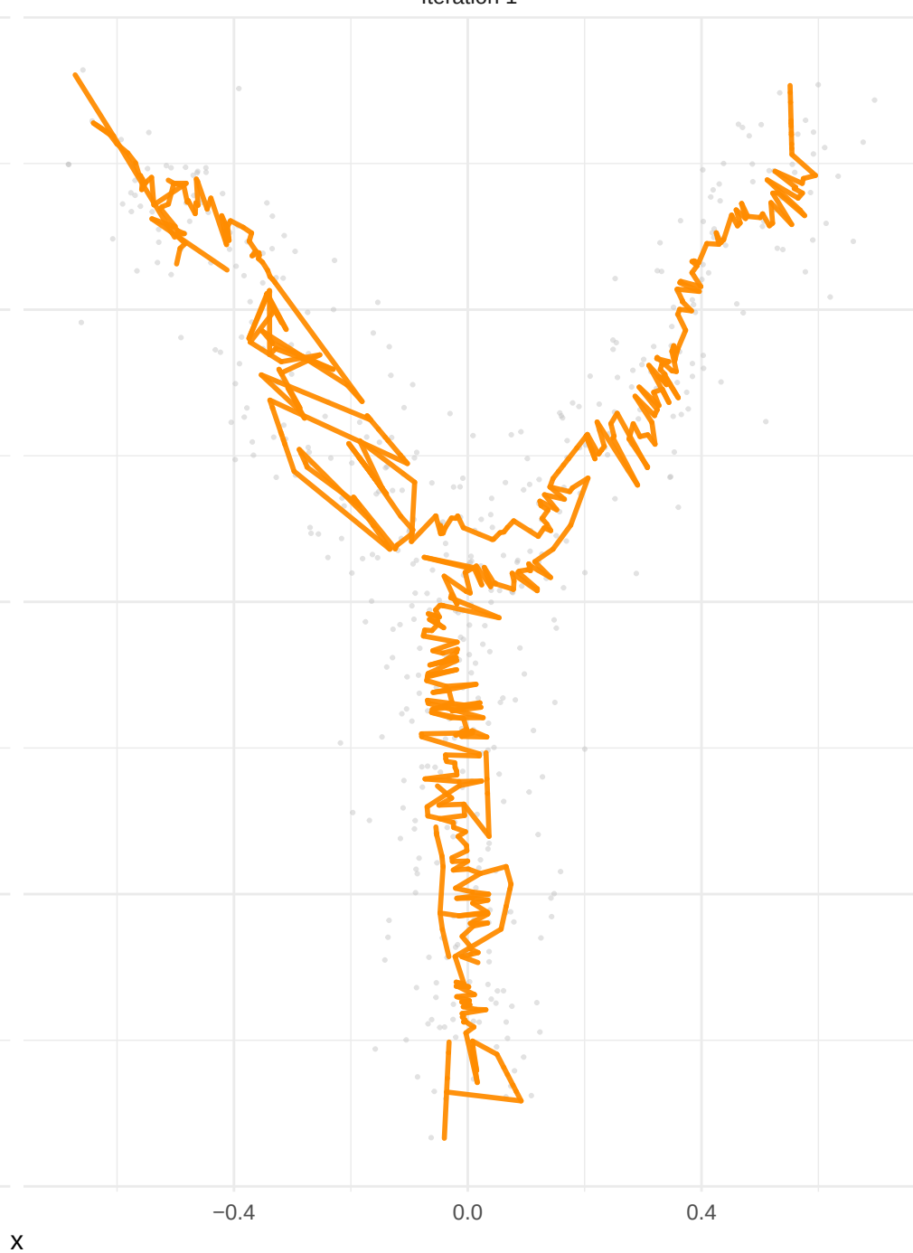
Iteration 1
