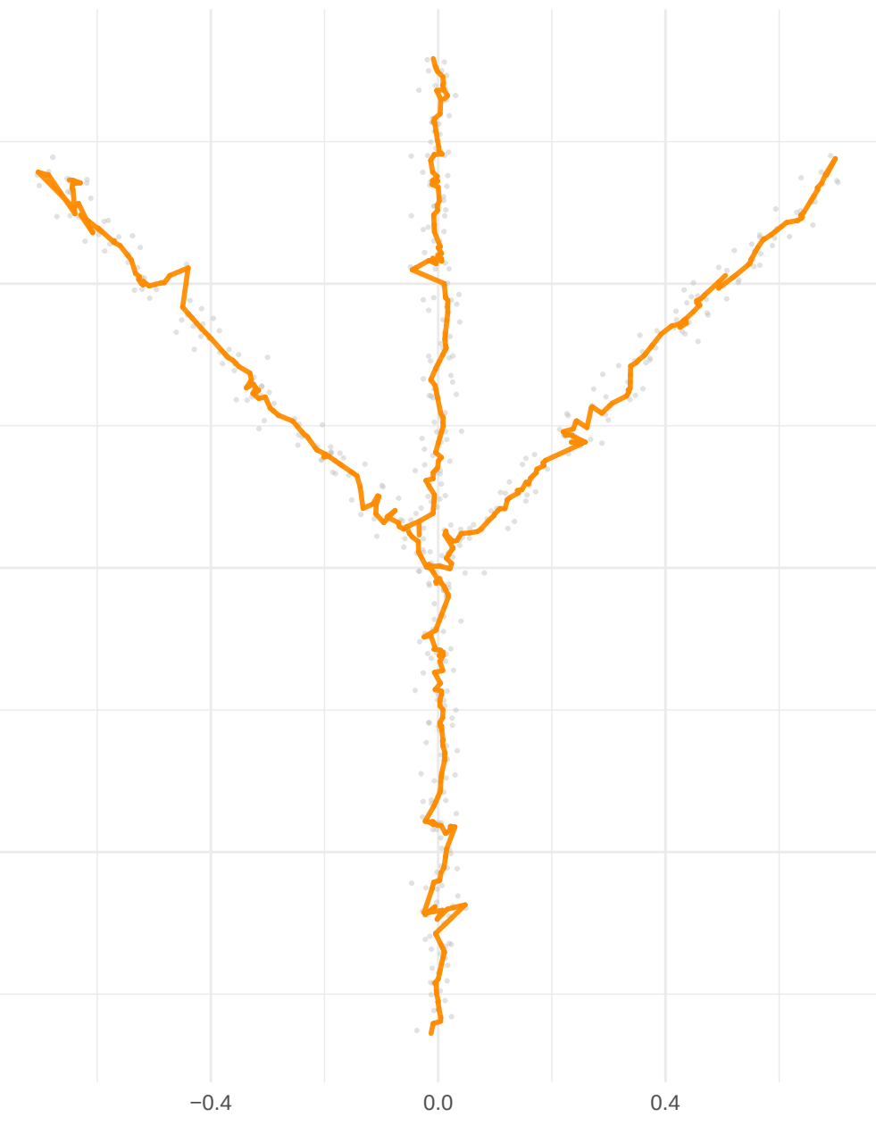
Iteration 1
