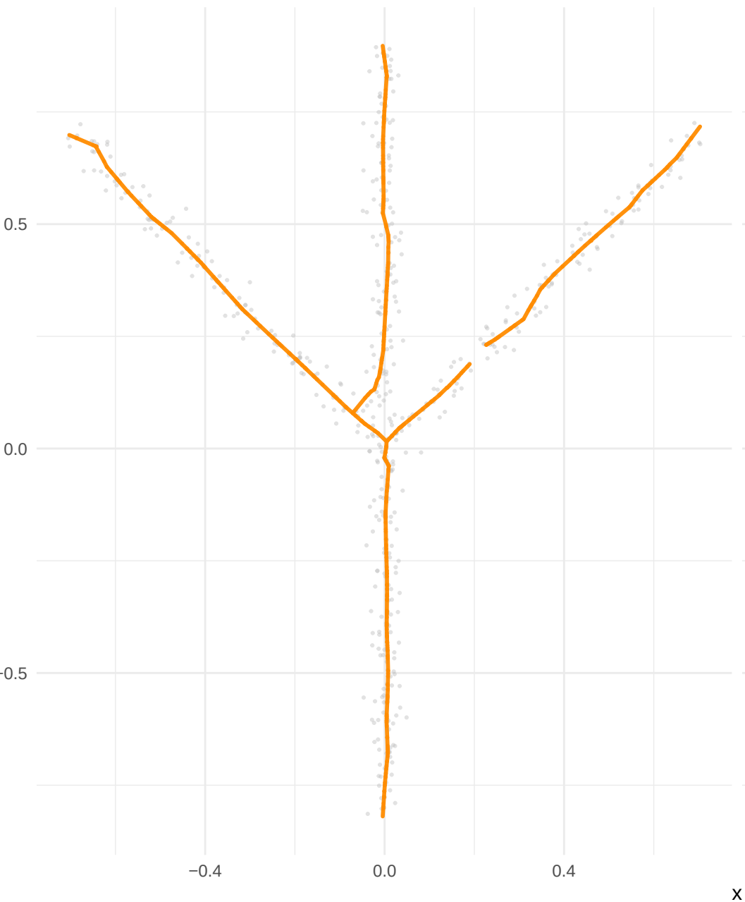
Final
