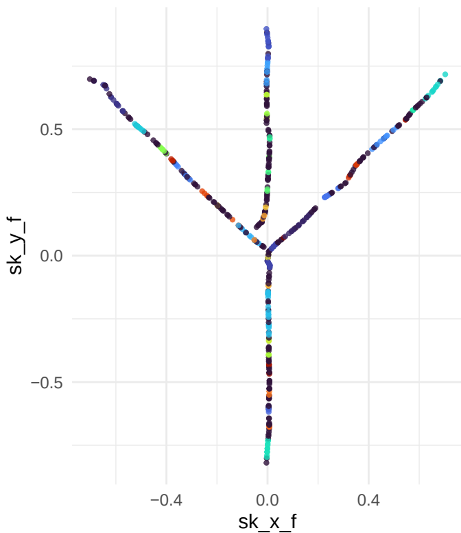
Converged
