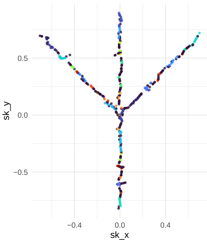
Iteration 1
