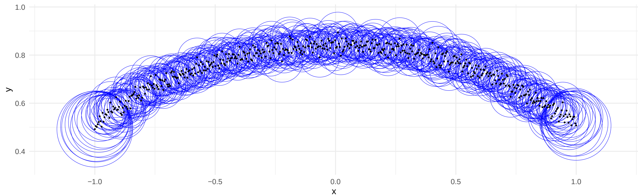
All Adaptive Spheres Visualizing local neighborhood size (radius) for every point.
