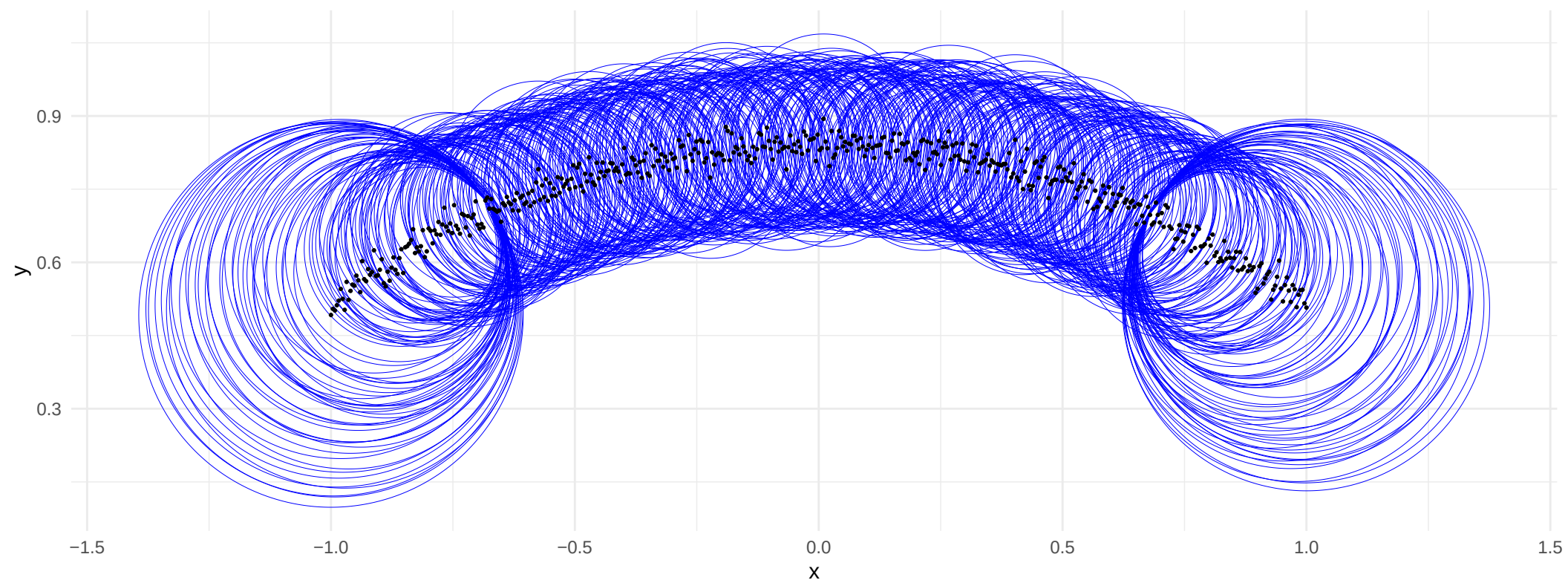
All Adaptive Spheres Visualizing local neighborhood size (radius) for every point.
