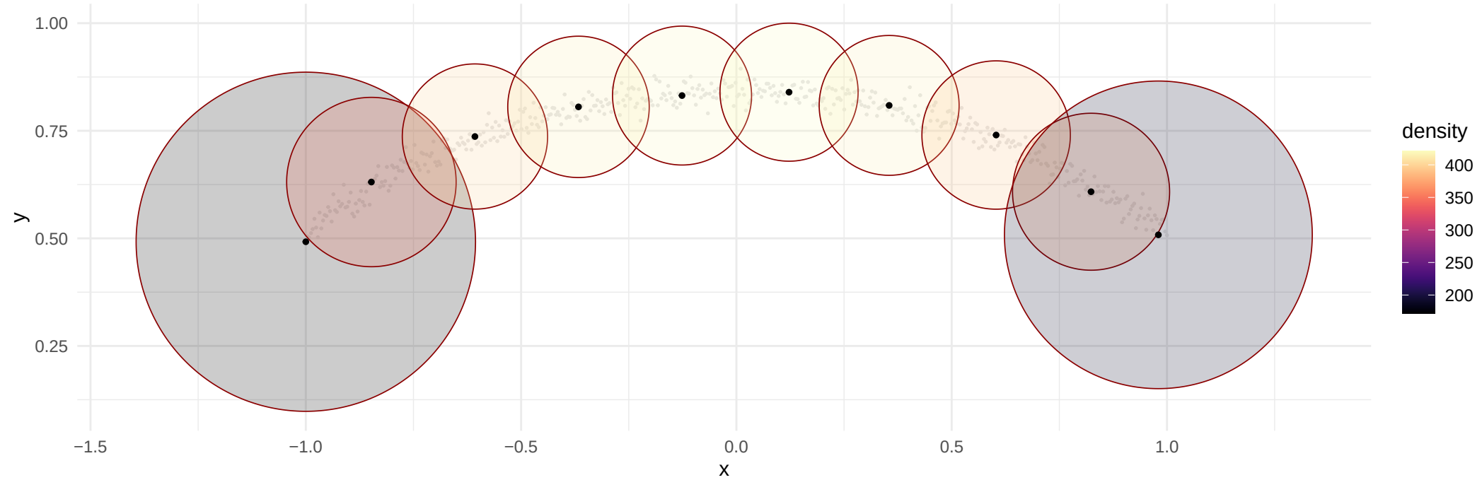
Atlas Selection (Anchors)
