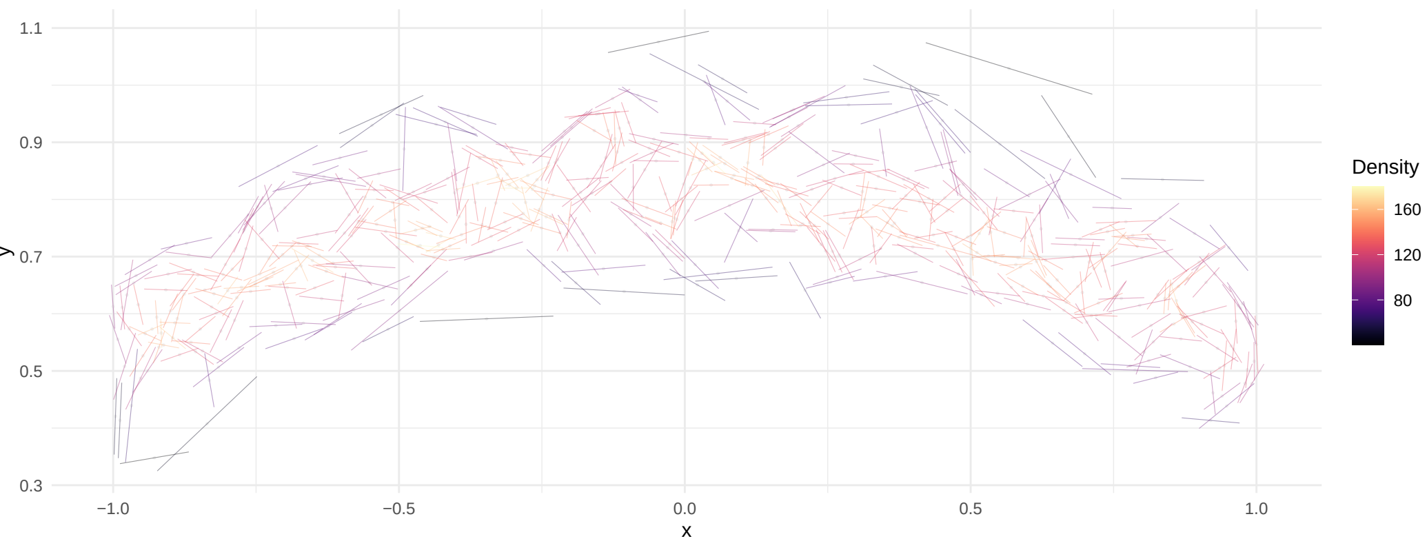
Global Tangent Field (PC1)
