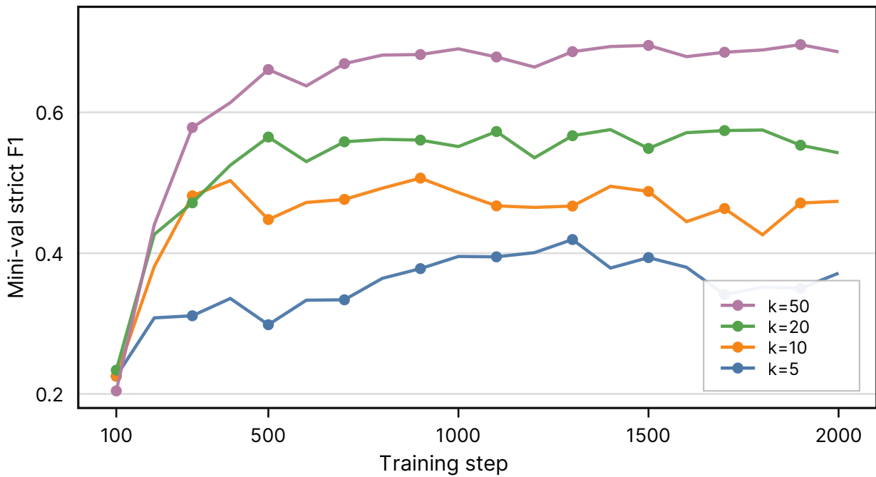
BART fitness curve
